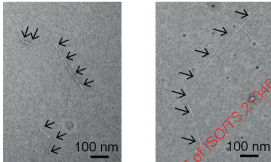
Figure A.9 — Examples of iCNF images for length measurement
