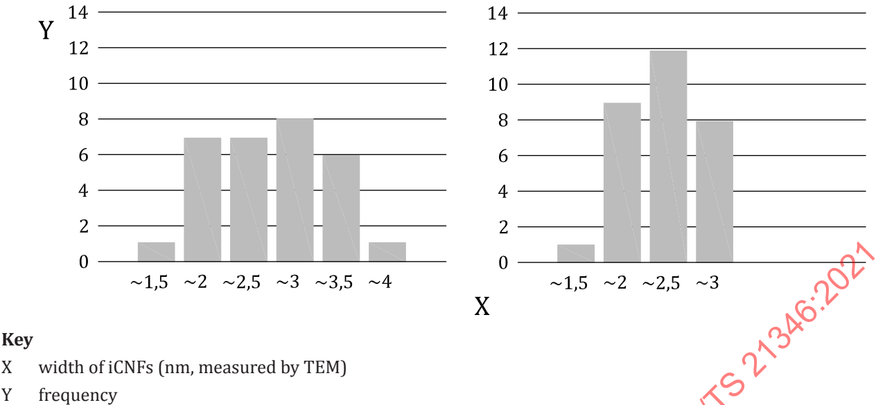
Figure A.7 — Examples of histograms for iCNF width distributions
