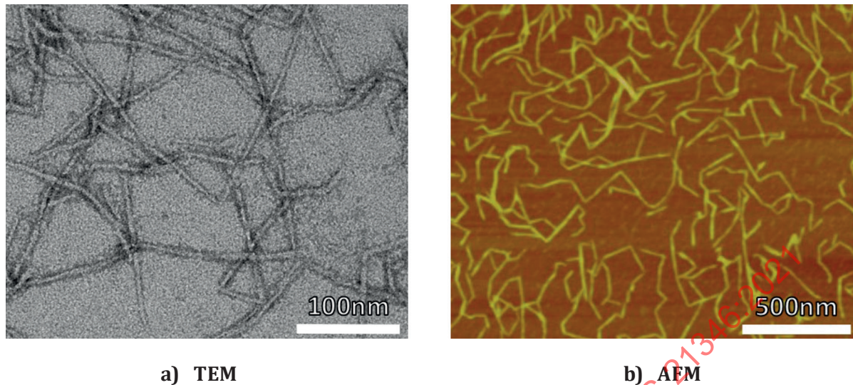
Figure A.1 — Images of iCNFs
