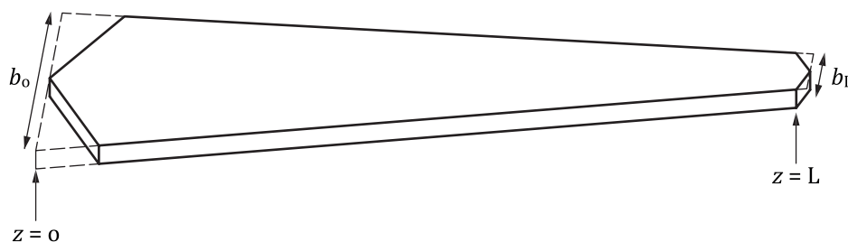
Figure 3 — Depiction of a trapezoidal channel geometry. Adapted from Litzen and Wahlund 1991 [26]
