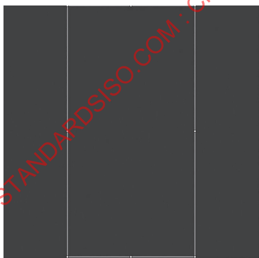
a) Averaging area for the horizontal direction on the background noise image I_{BG2} b) Vertical line profile L_{pVA} of the horizontally averaged noise
