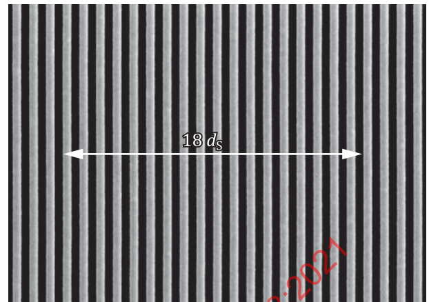
b) Pitch of the RM: d = 500 nm. Total number of pitches: n_p = 18 Image Magnification setting: M = 12\,000 . Accelerating voltage: V_a = 1 kV
