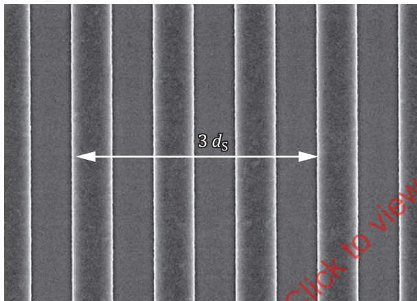
c) Pitch of the RM: d = 1\,000 nm. Total number of pitches: n_p = 3 Image Magnification setting: M = 30\,000 . Accelerating voltage: V_a = 15 kV
