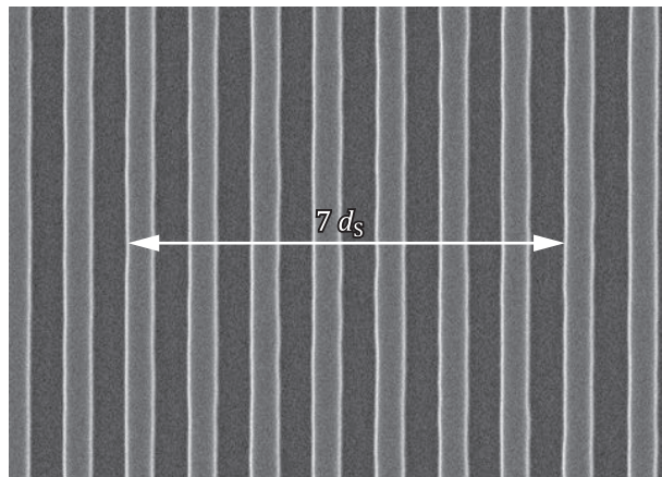
a) Pitch of the RM: d = 100 nm. Total number of pitches: n_p = 7 Image Magnification setting: M = 150\,000 . Accelerating voltage: V_a = 15 kV
