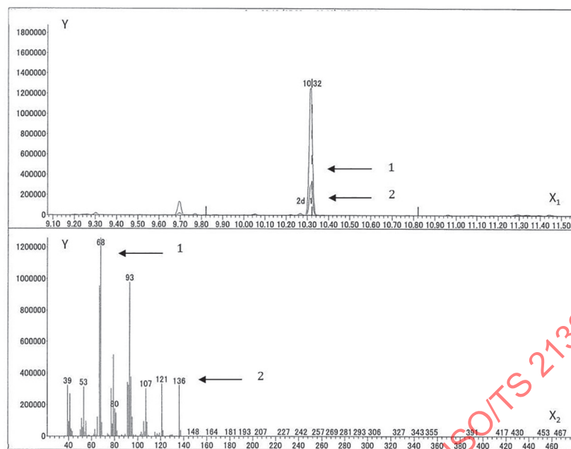
a) IpD peak from IR calibration standard
