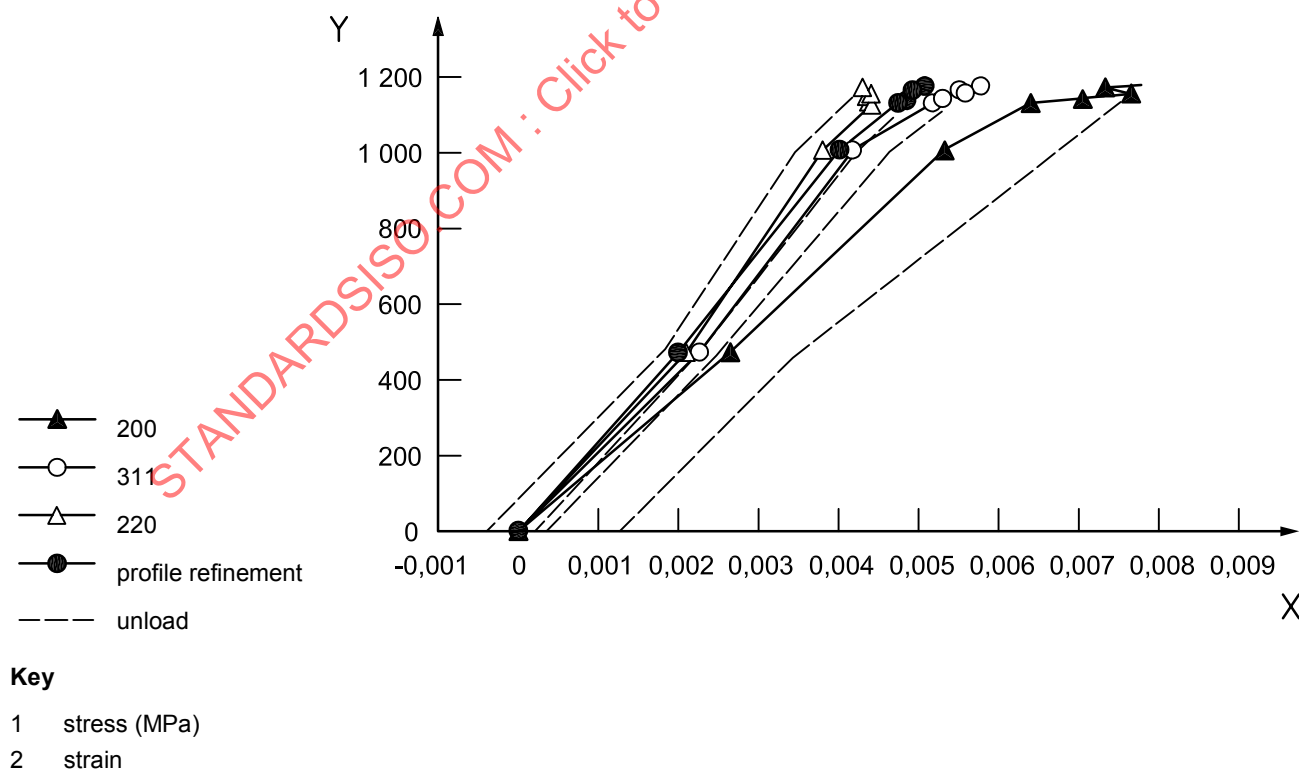
Figure 7 — Effect of yielding on response of different crystallographic planes to loading and unloading of a tensile bar of a nickel alloy [2]
