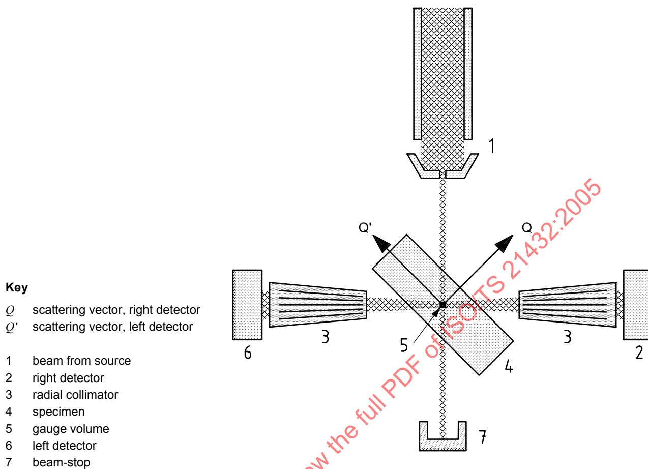
Figure 4 — Schematic illustration of a pulsed-source TOF diffractometer for strain measurement
