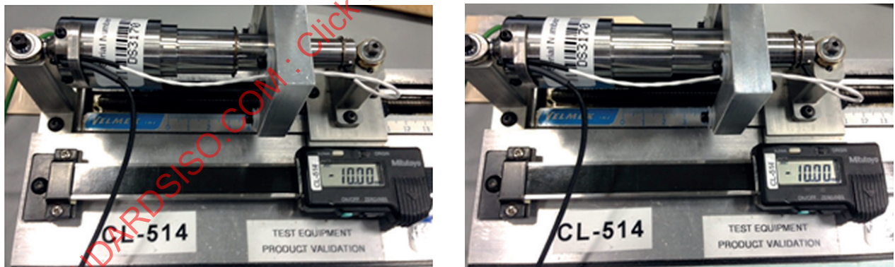
Figure 4 — IR-TRACC tubes-in shown left and tubes-out shown right
