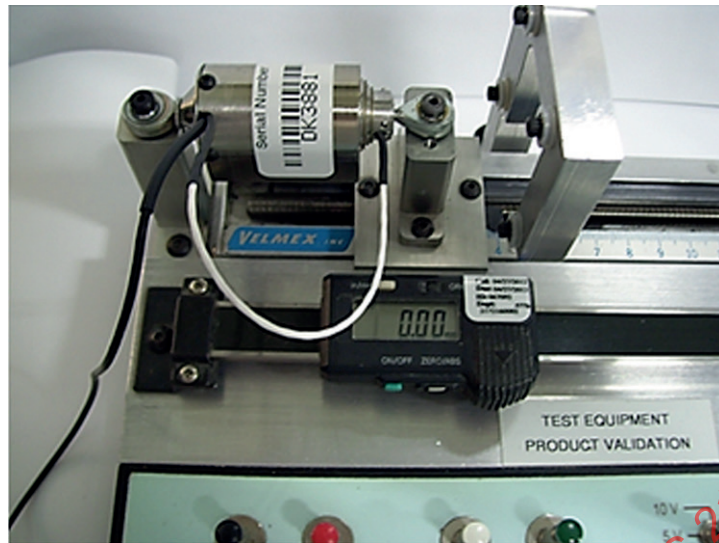
Figure 2 — IR-TRACC fully collapsed
