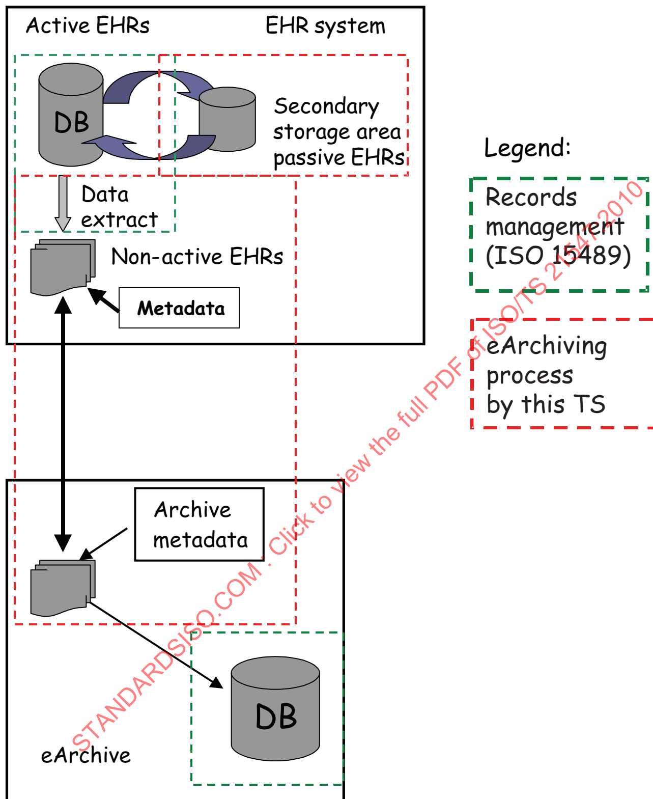
Figure 5 — Areas covered by the eArchiving process
