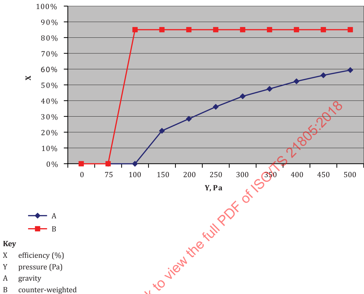
Figure 5 — Efficiency of pressure-relief vents
