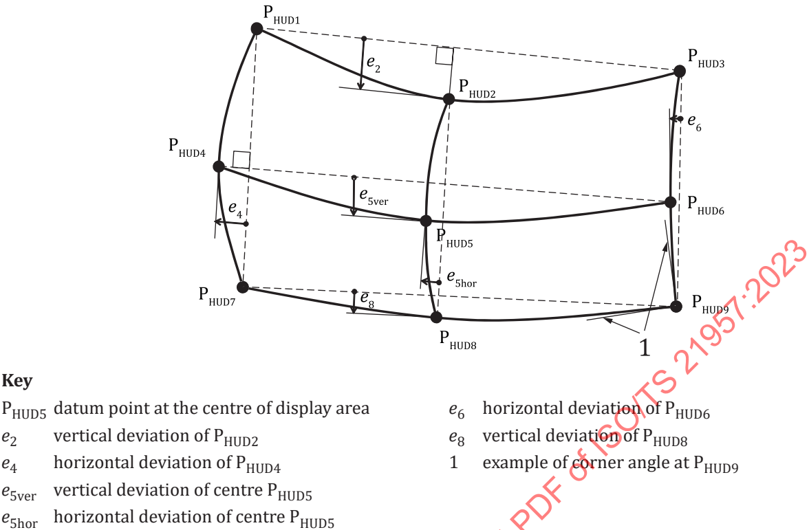
Figure 24 — Distortion measuring reference points
