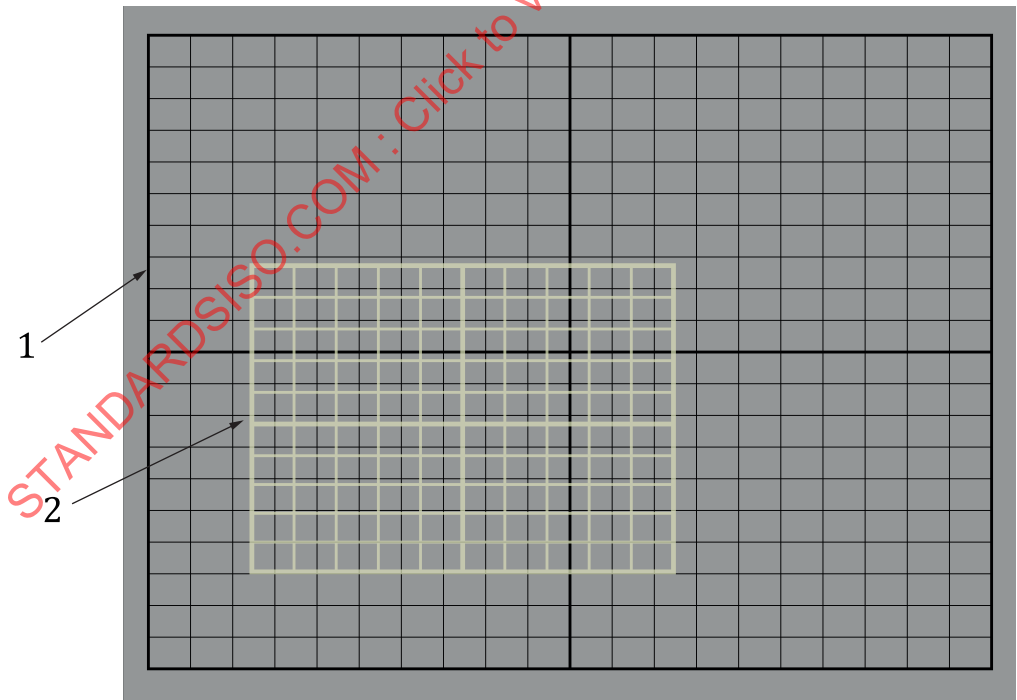
Figure 14 — Conceptual image of an in-focus HUD frame and out-of-focus grid screen chart
