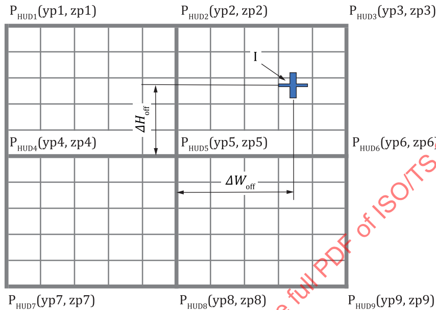
Figure 18 — Image outer frame coordinate and datum
