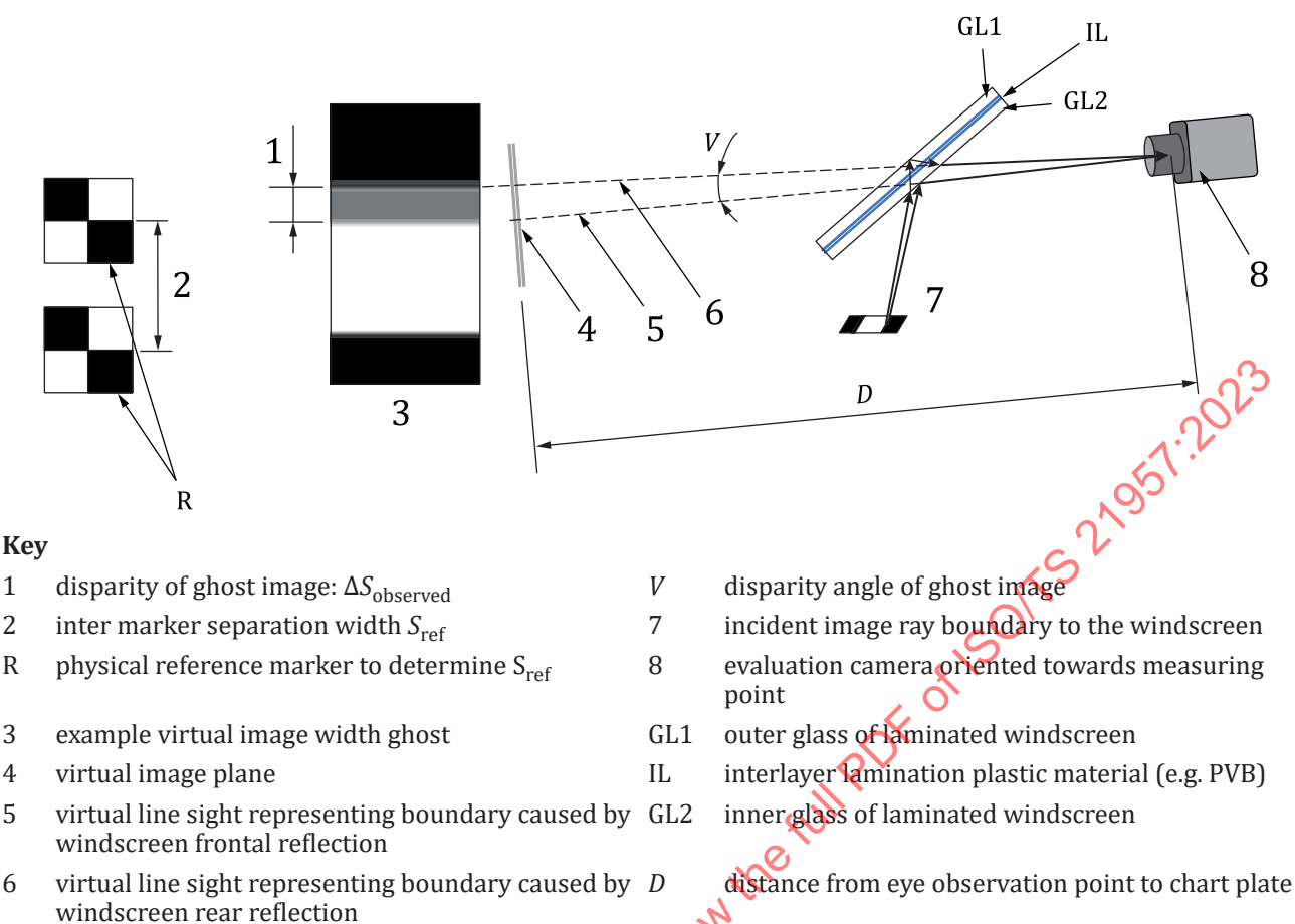
Figure 22 — Conceptual cross-sectional view to measure ghost width
