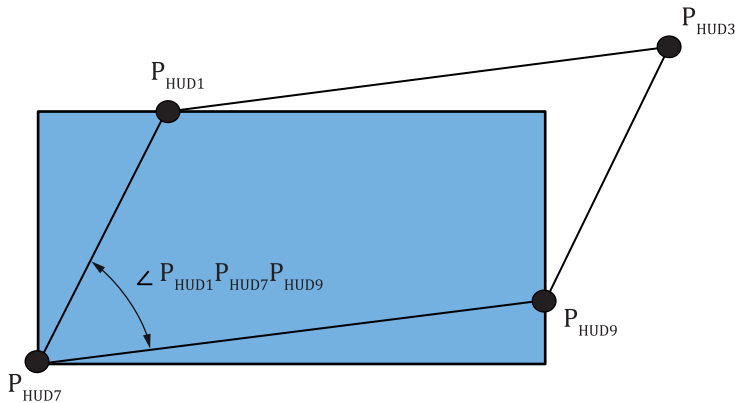
Figure 26 — Distortion measuring points
