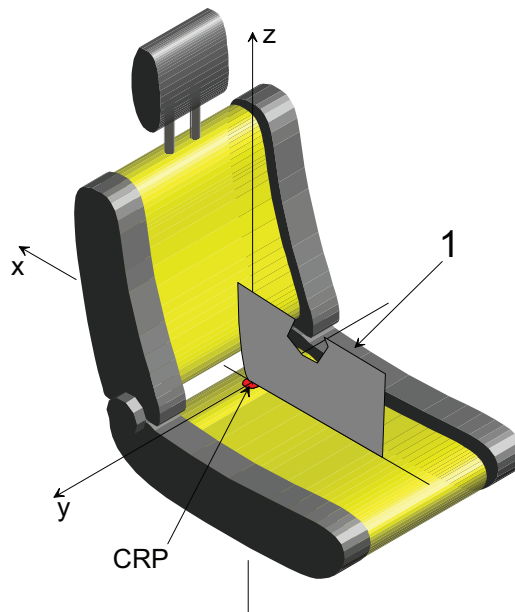
Figure B.4 — Reference co-ordinate system
