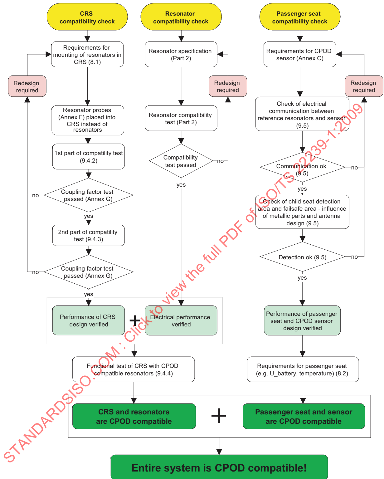
Figure 2 — Main steps for obtaining CPOD compatibility of the entire system
