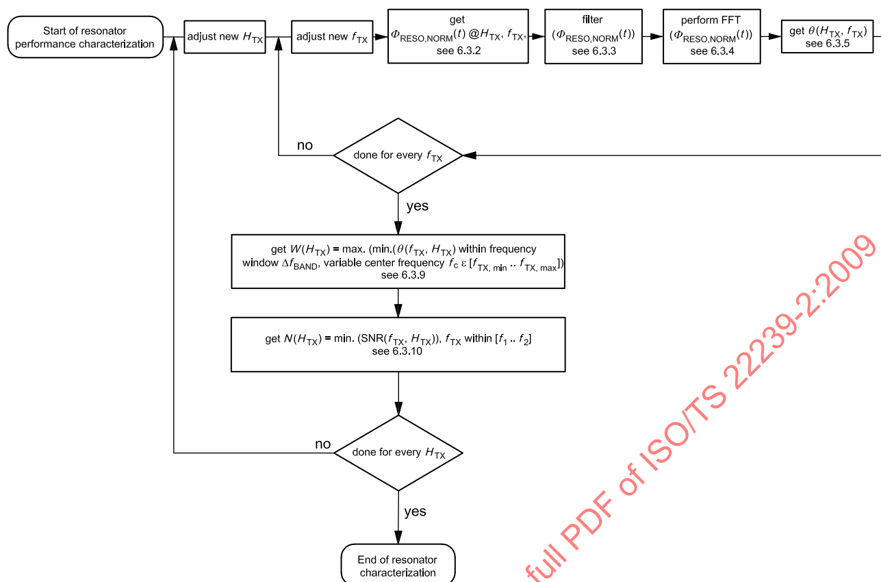
Figure 8 — Procedure to derive W(H_{TX}) and N(H_{TX}) for magnetic field strength H_{TX}
