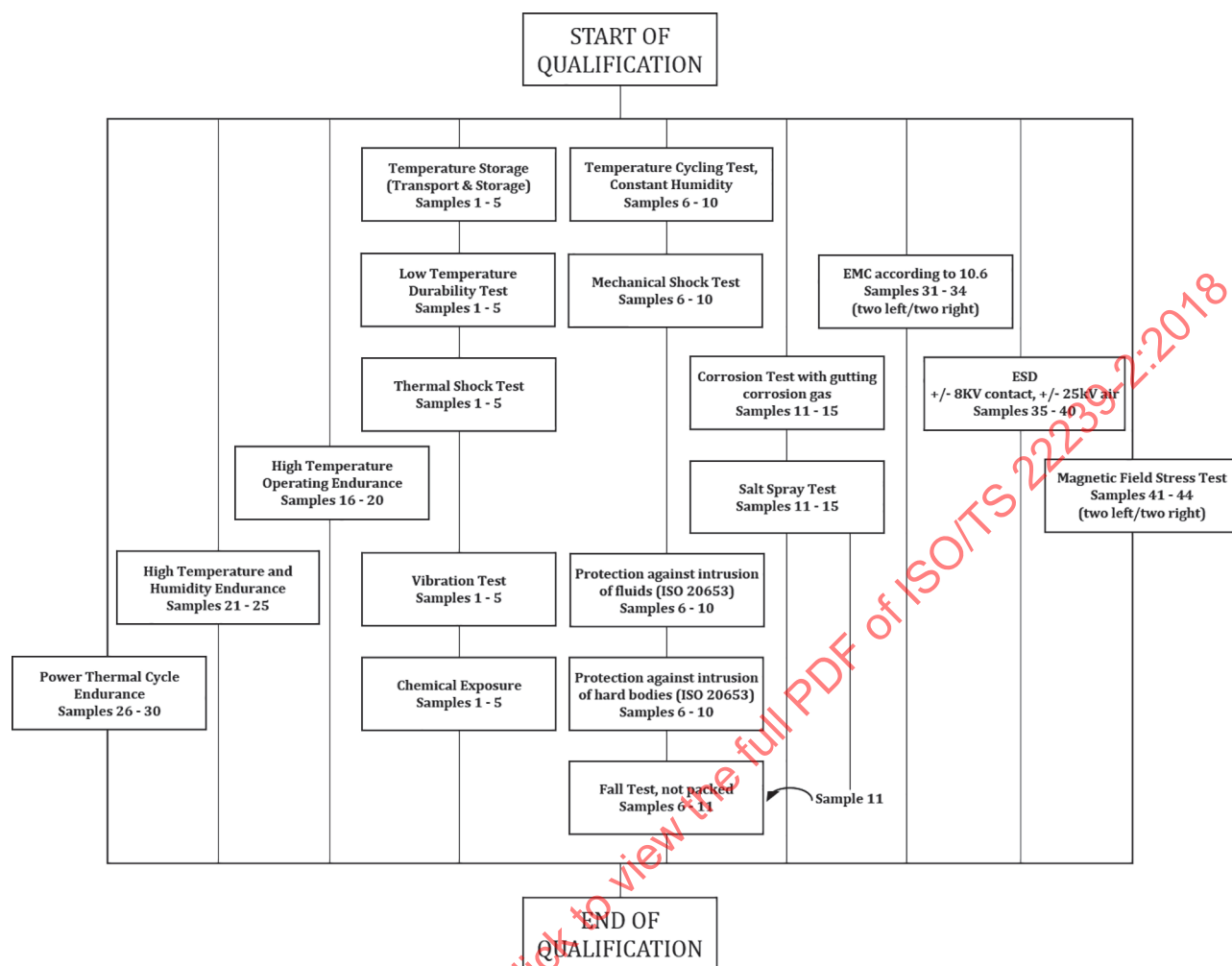
Figure 36 — Qualification flow chart
