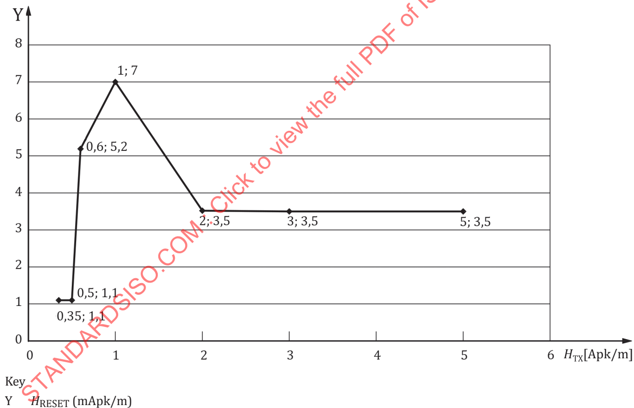
Figure 21 — H_{\text{RESET}} versus magnetic field strength, H_{\text{TX}}
