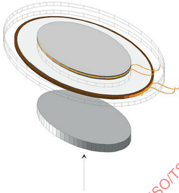
Figure A.4 — Resonator compatibility test set-up antenna structure (bottom view)
