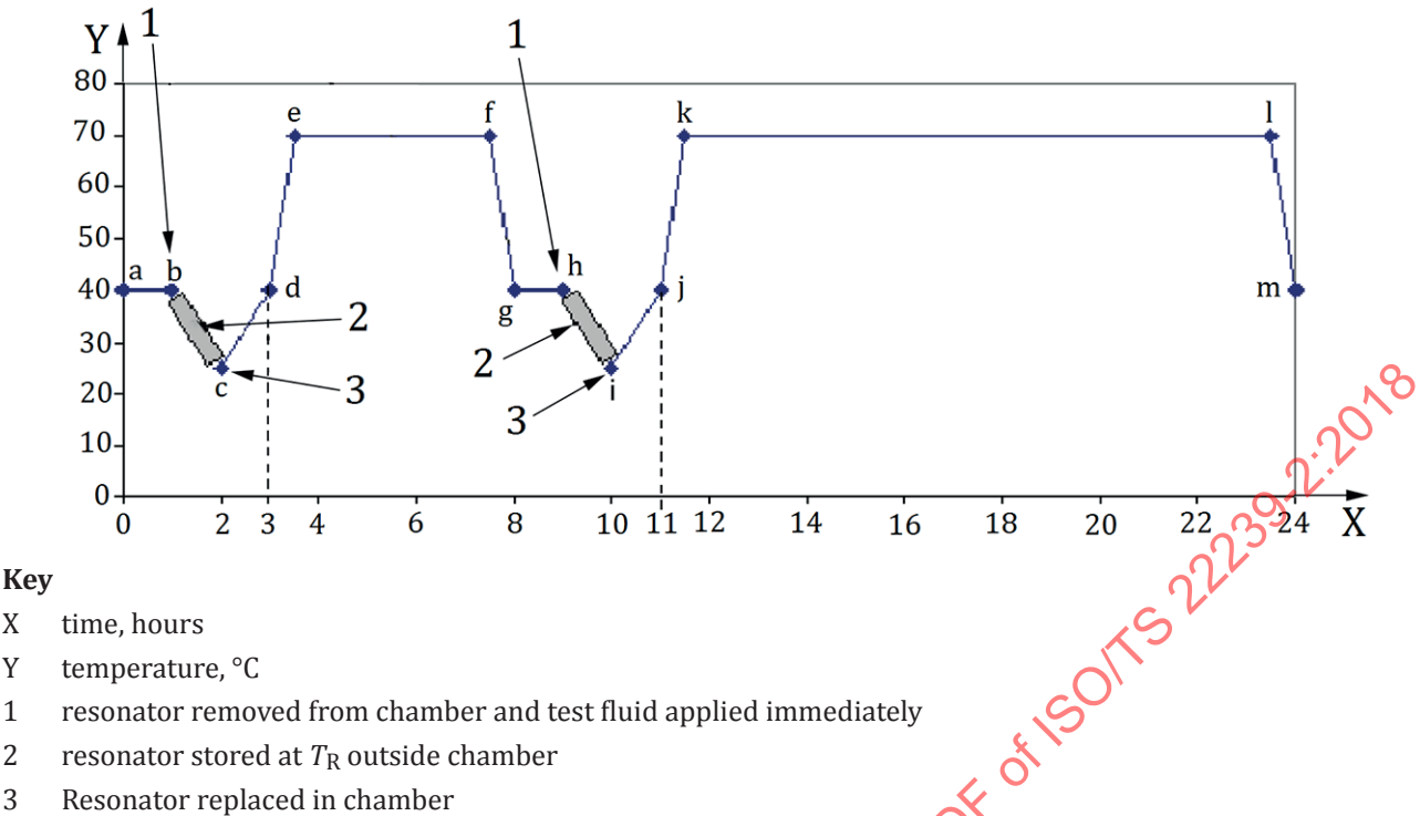
Figure 26 — Temperature profile (fluid exposure tests)
