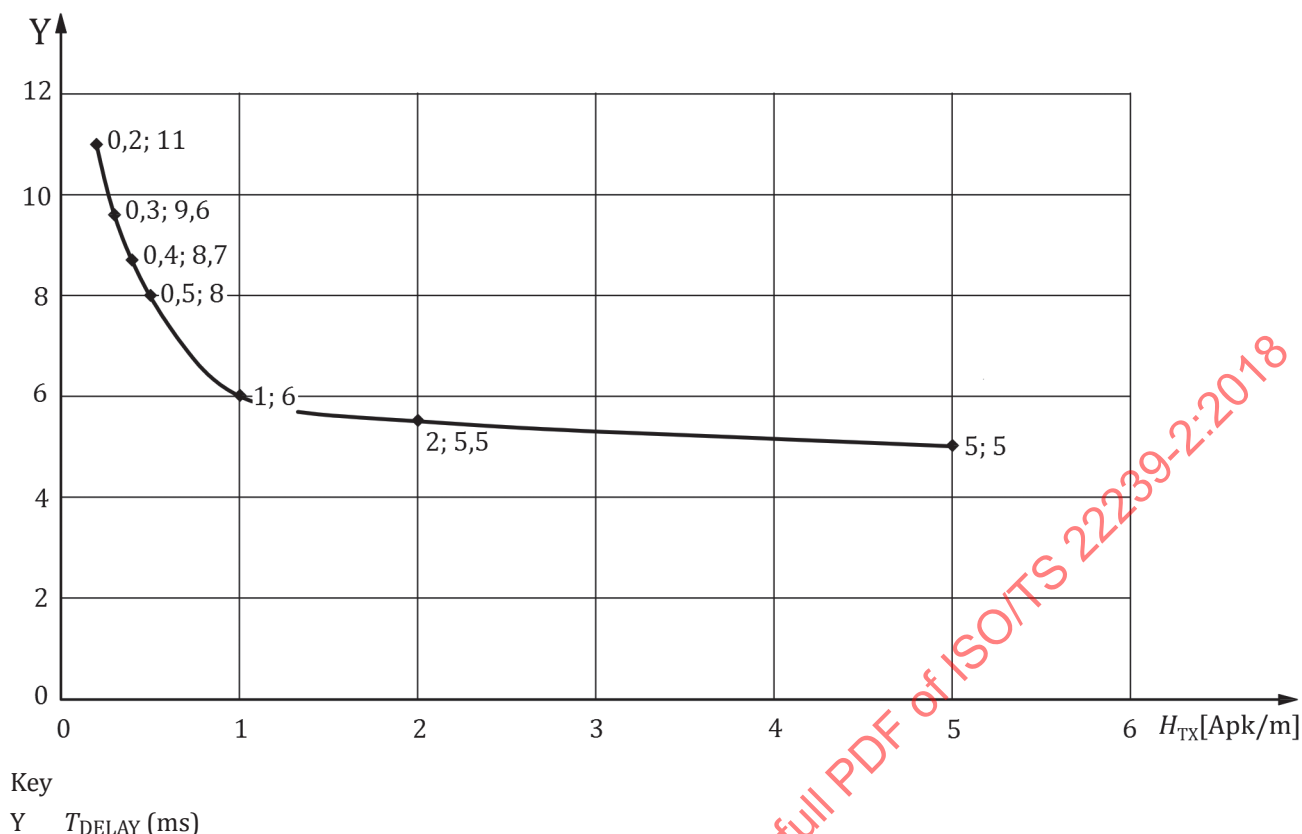
Figure 22 — T_{\text{DELAY}} versus magnetic field strength, H_{\text{TX}}
