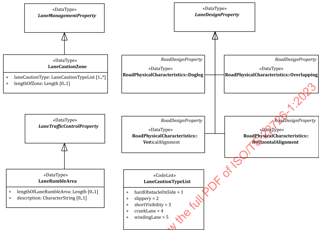
Figure 17 — Class diagram of LaneBeltSegmentProperty
