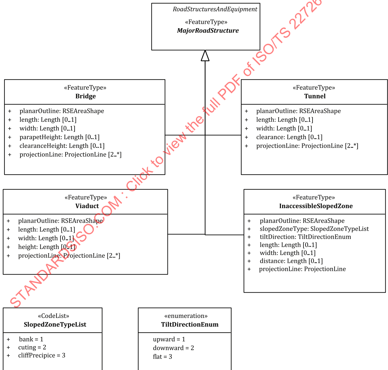
Figure 19 — MajorRoadStructure sub-package
