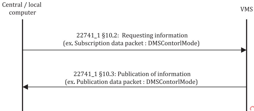
Figure 2 — Procedure to get elemental data
