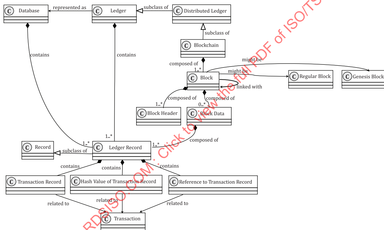
Figure 3 — DLT ontology diagram - Graphical overview
