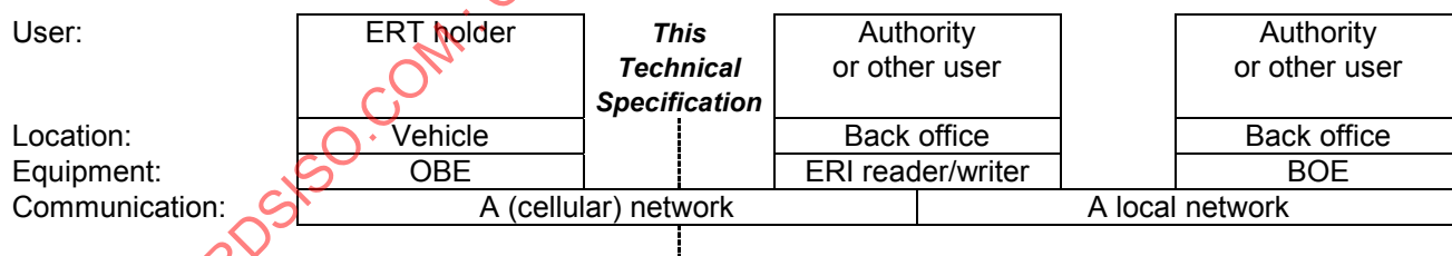
Figure 7 — Overall remote communication concept
