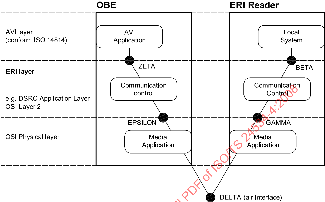
Figure 10 — The location of the ERI layer in the ISO 14814 reference architecture
