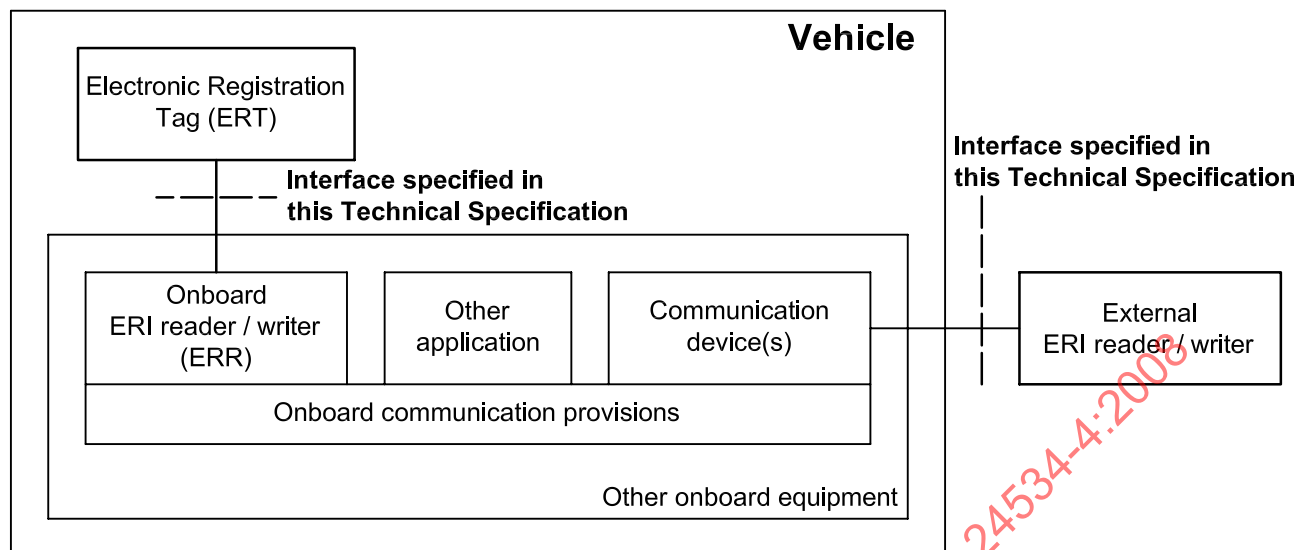
Figure 1 — System concept and supported interfaces
