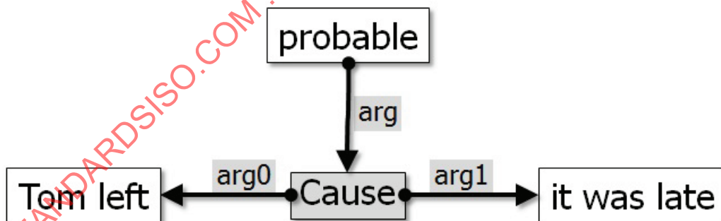
Figure 5 — Content structure of (4)
