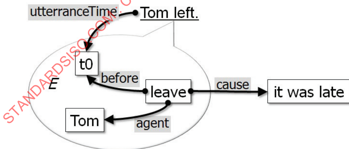
Figure 3 — Segment 'Tom left.' and detailed content structure
