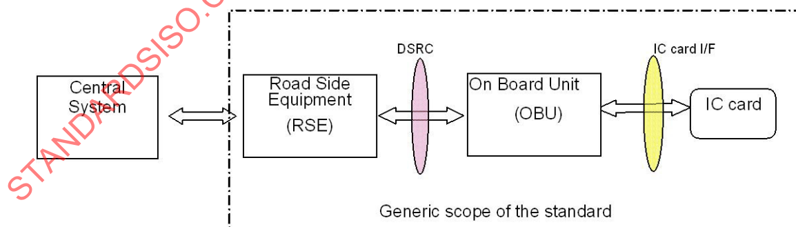
Figure 3 — Configuration of on-board account and generic scope of ISO/TS 25110
