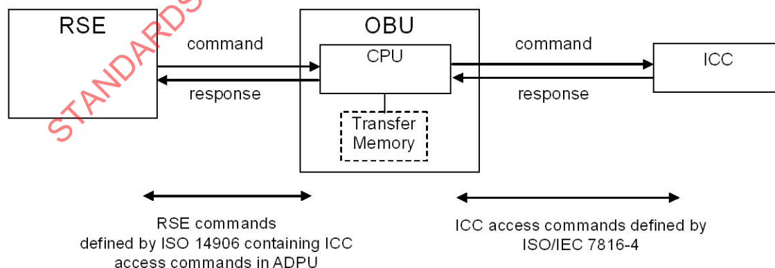
Figure 12 — Functional configuration of transparent type
