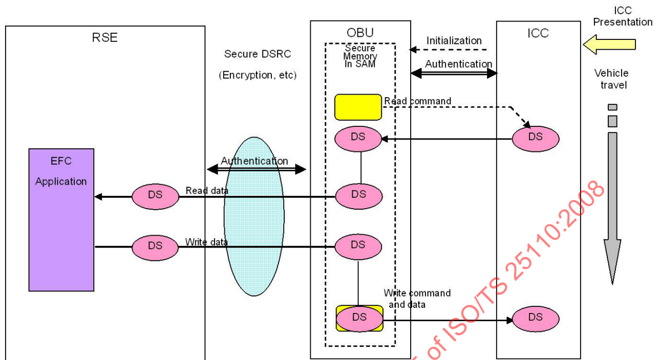
Figure 10 — Data transfer process of caching type
