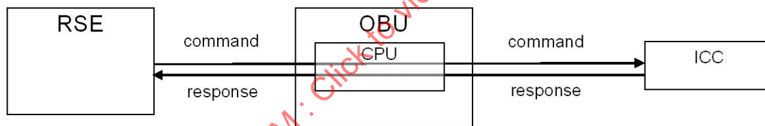
Figure 5 — Generic structure of transparent type
