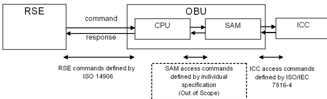
Figure 13 — Functional configuration of caching type
