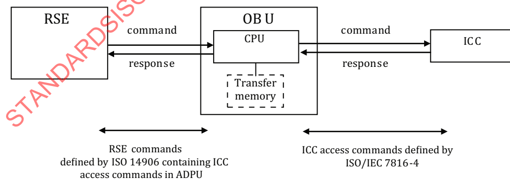
Figure 12 — Functional configuration of transparent type
