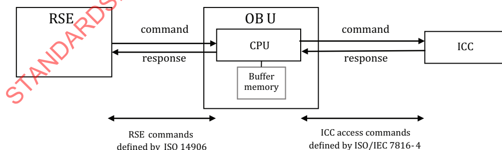
Figure 14 — Functional configuration of buffering type
