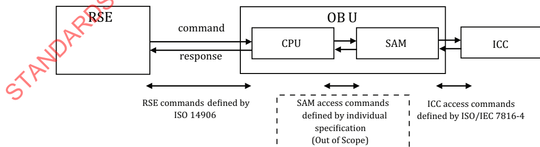
Figure 13 — Functional configuration of caching type
