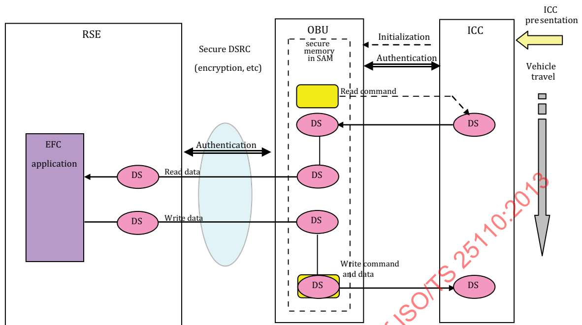
Figure 10 — Data transfer process of caching type
