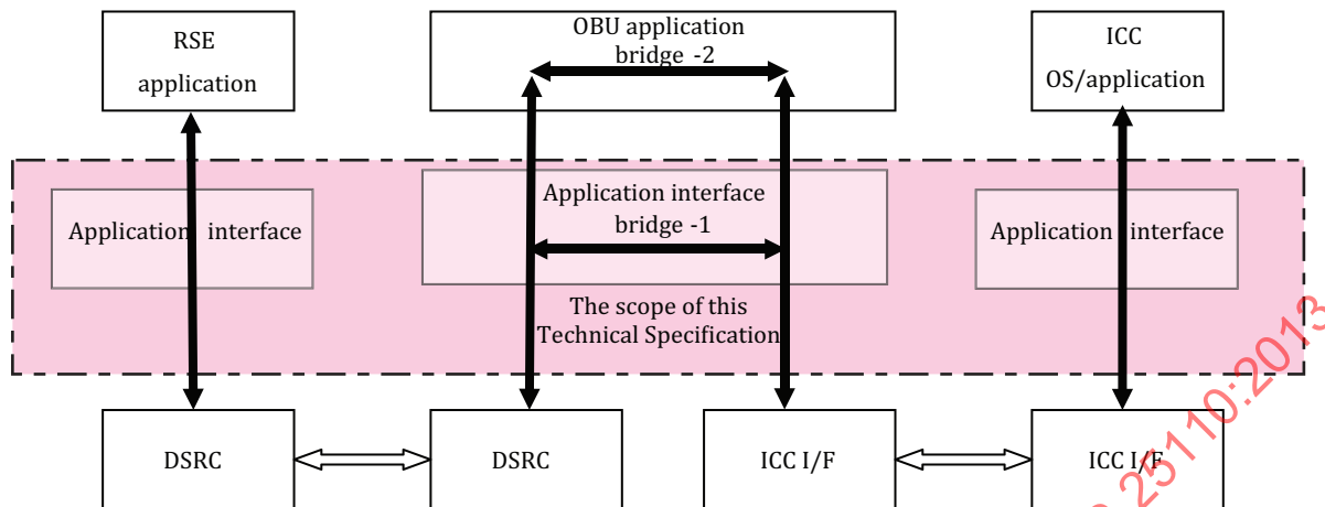
Figure 4 — Scope of ISO/TS 25110
