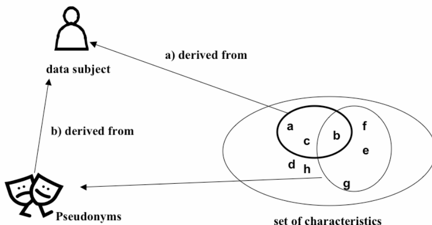
Figure 5 — Reversible pseudonymization
