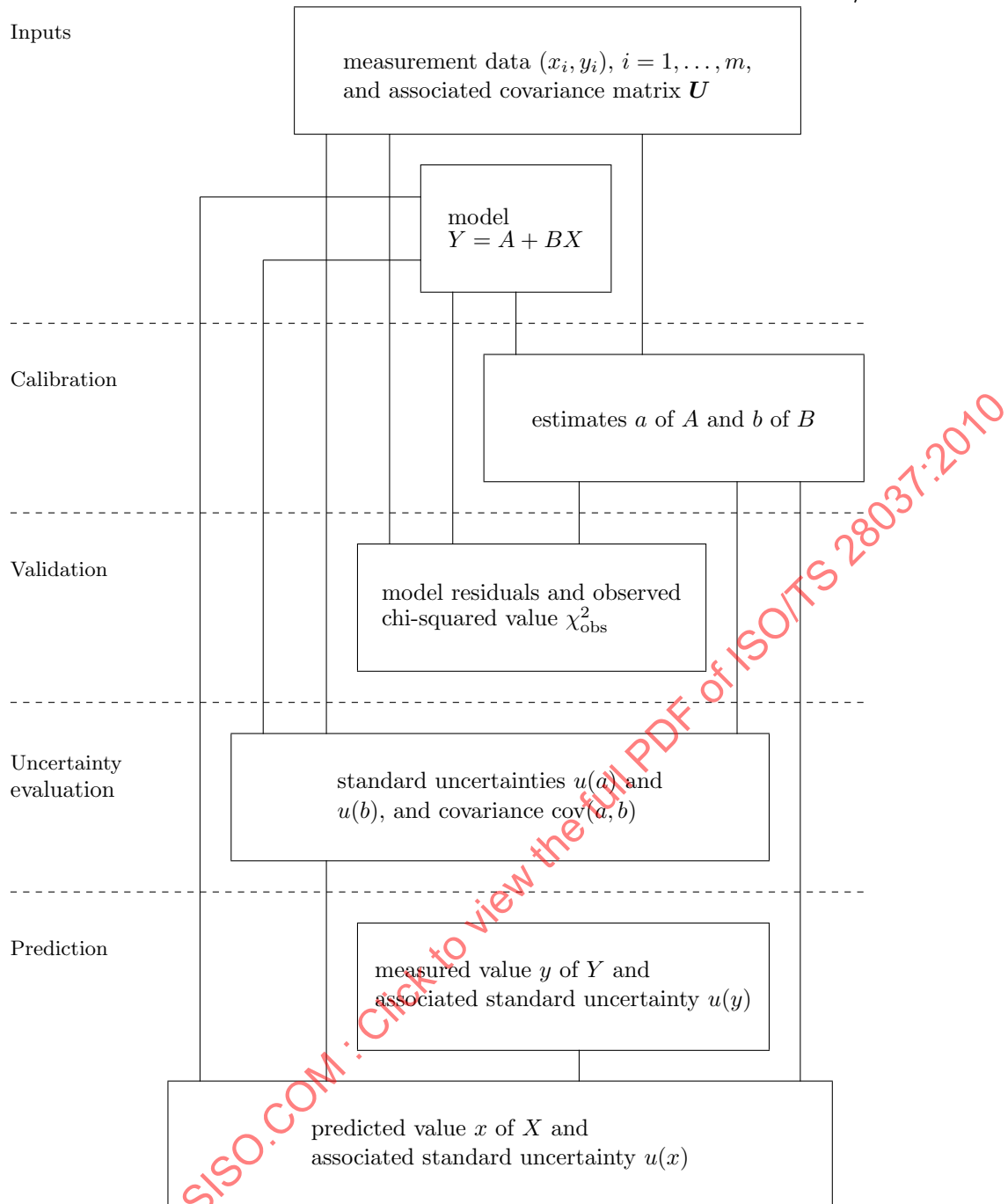
Figure 1 — Summary of the steps in the determination and use of straight-line calibration functions
