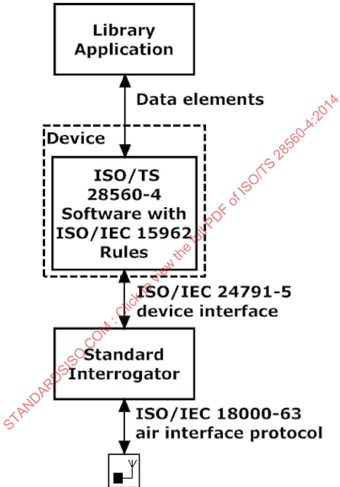
Figure 2 — Architecture with integrated data element software component
