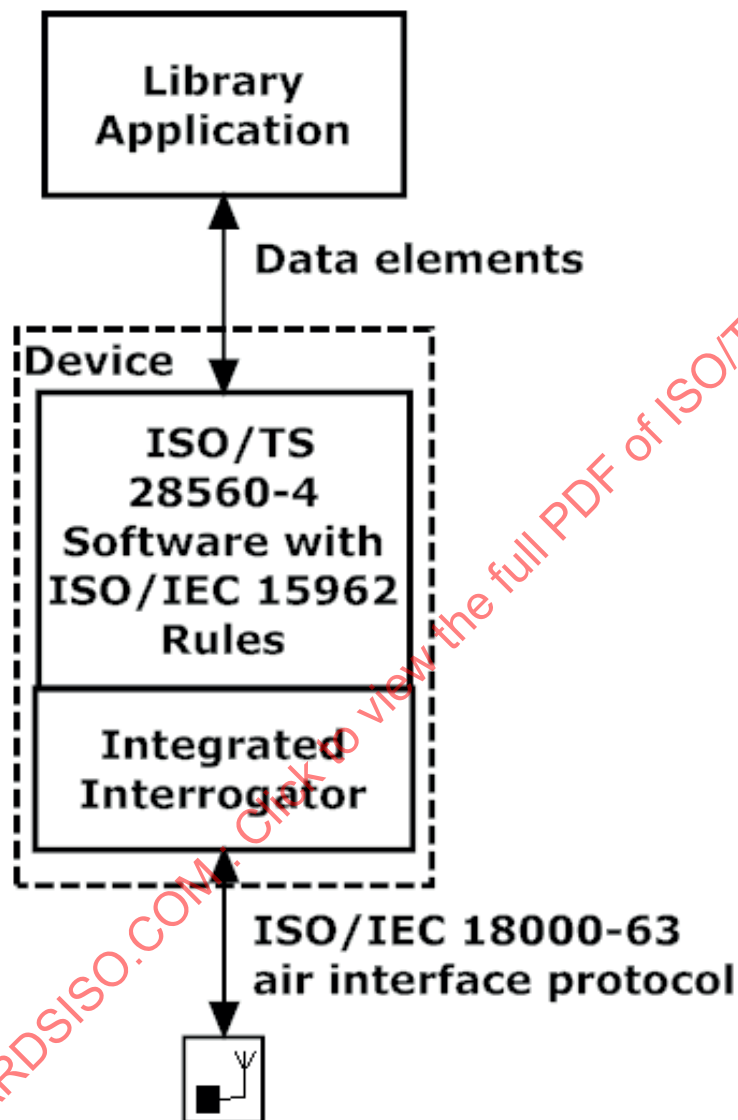
Figure 3 — Legacy-based architecture
