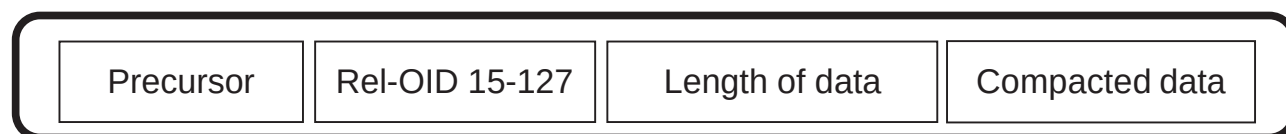
Figure 7 — ISO/IEC data set with Relative-OID values 15 to 127
