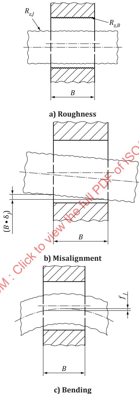
Figure 1 — Influences on the minimum permissible lubricant film thickness
