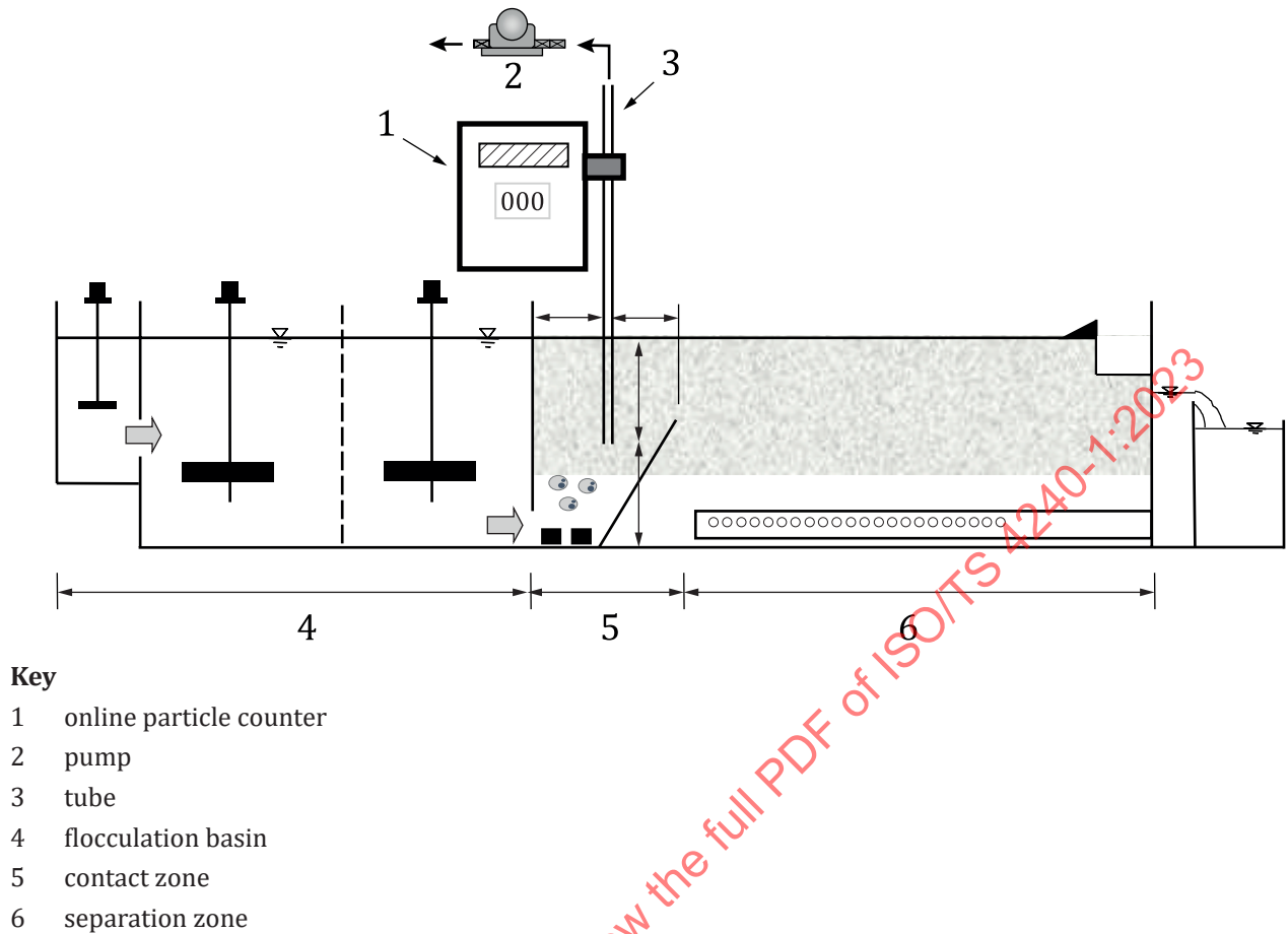
Figure 1 — Schematic diagram of equipment for BVC evaluation
