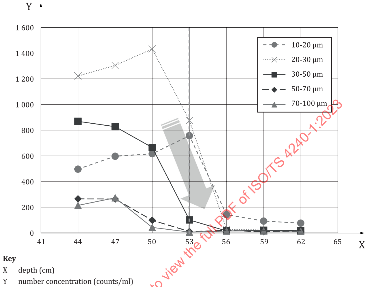
Figure C.1 — Particles and bubble counts with depth in a pilot plant
