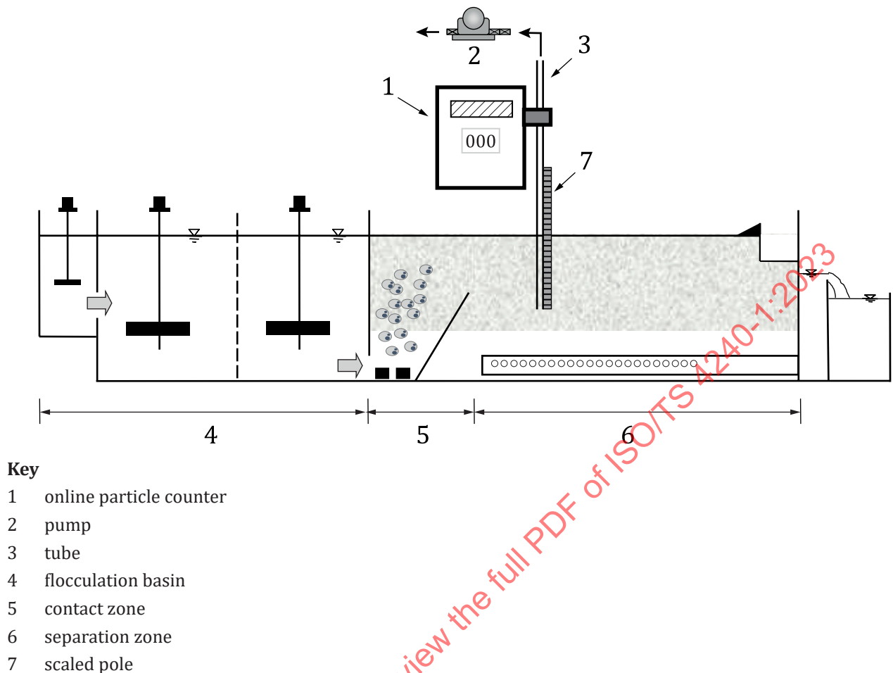
Figure 2 — Schematic diagram of equipment for bubble bed depth measurement
