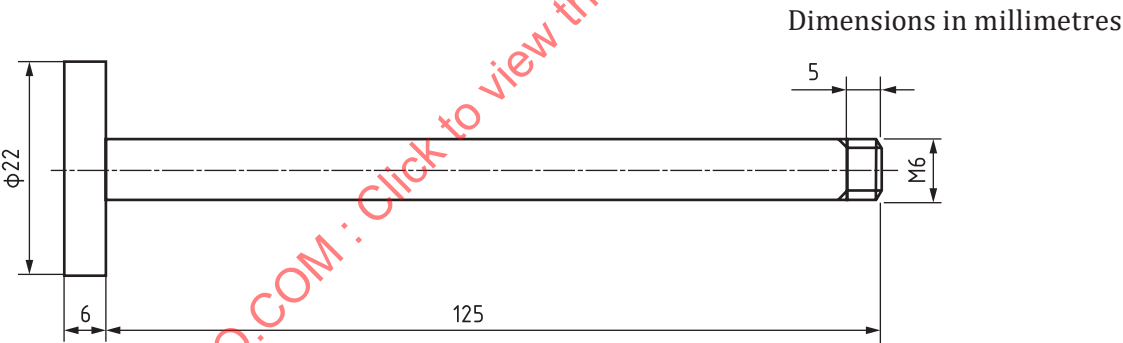
Figure A.1 — Jigs and alignment for Kemper and Killian's test method
