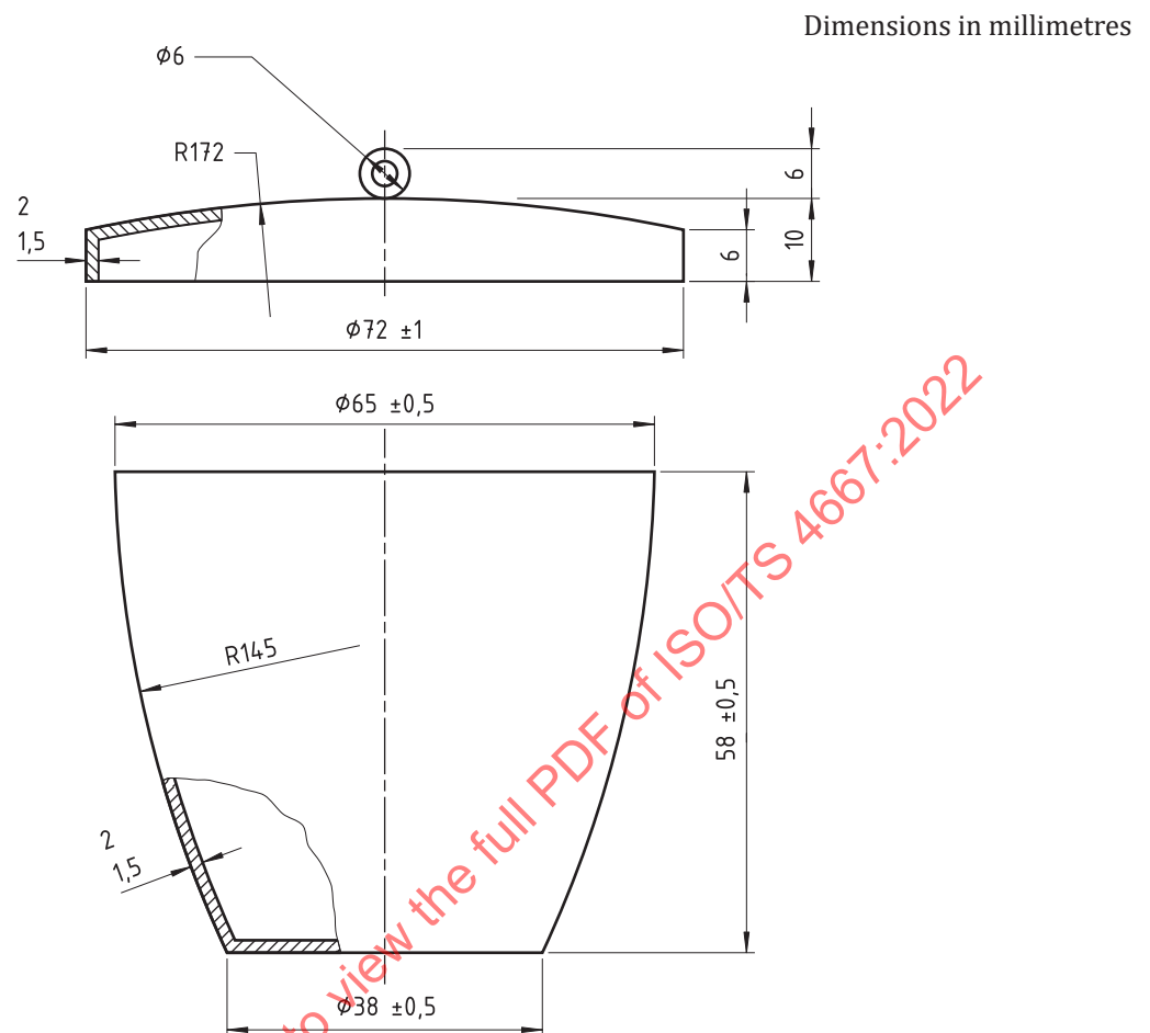
Figure 1 — Schematic of the crucible and lid
