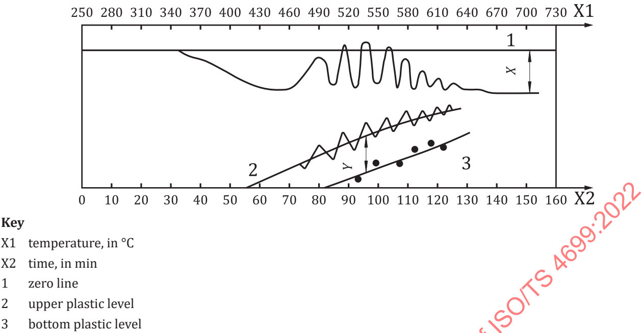
Figure 9 — Schematic diagram of plastic layer curve
