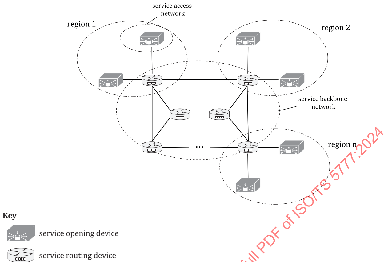
Figure 5 — Mesh topology
