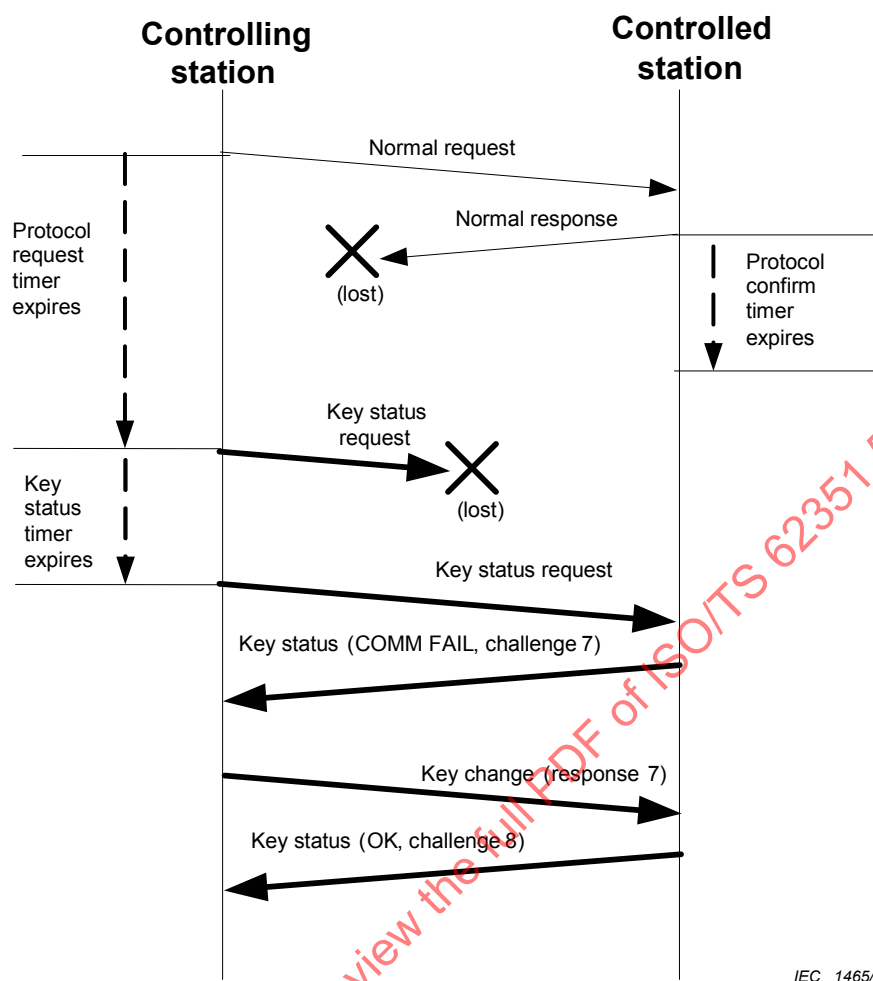
Figure 6 – Example of communications failure followed by session key change
