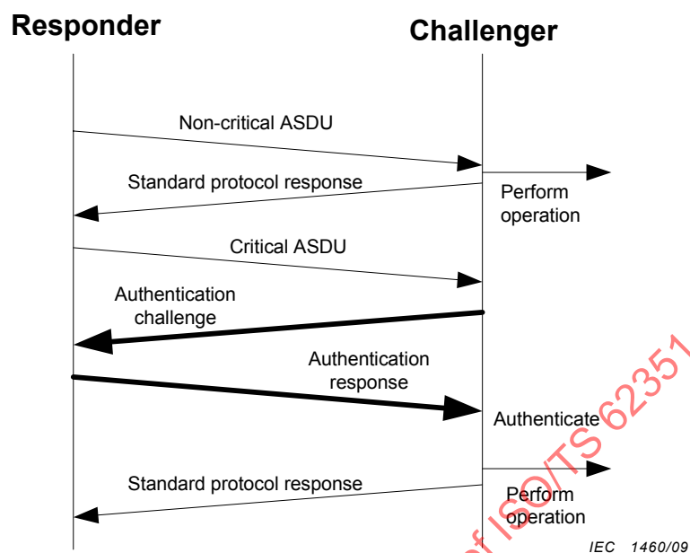
Figure 1 – Example of successful challenge of critical ASDU
