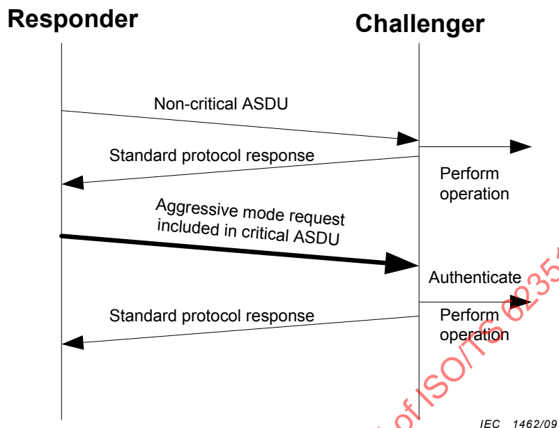
Figure 3 – Example of a successful aggressive mode request
