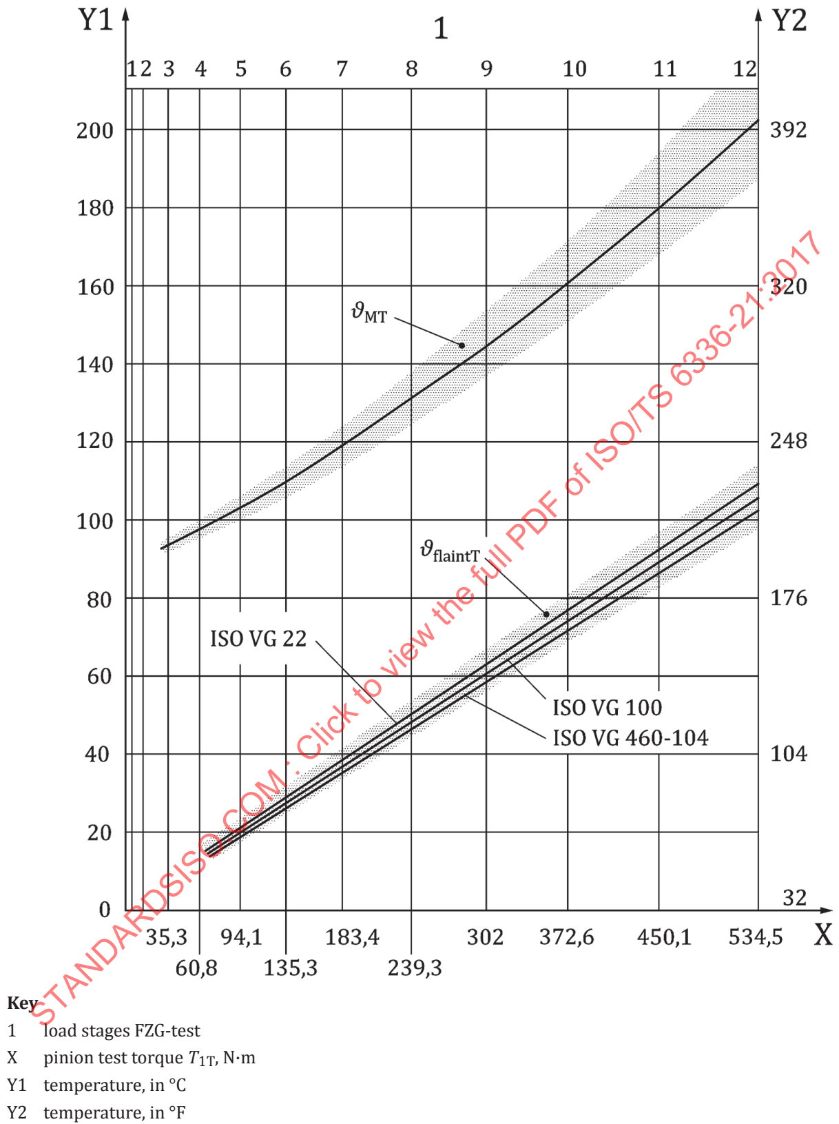
Figure 9 — Scuffing temperature, \vartheta_{intS} , for the FZG test A/8,3/90
