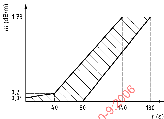
Figure 16 — Limits for m against time, t , Fire TF4
