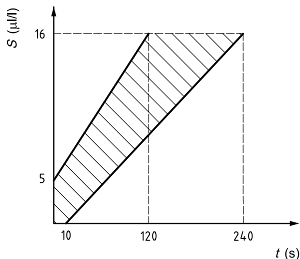
Figure 20 — Limits for S against time, t , Fire TF5
