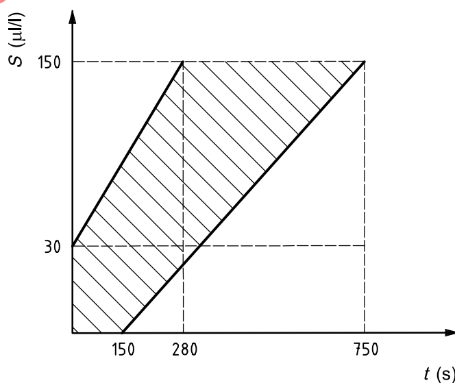
Figure 14 — Limits for S against time, t , Fire TF3
