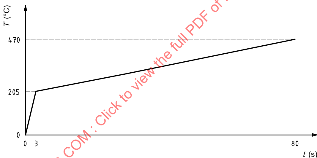
Figure 22 — Slow smouldering (pyrolysis) wood fire hotplate temperature vs. time
