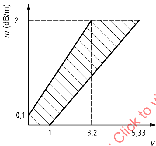
Figure 12 — Limits for m against y , Fire TF3
