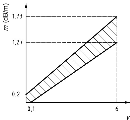
Figure 15 — Limits for m against y , Fire TF4
