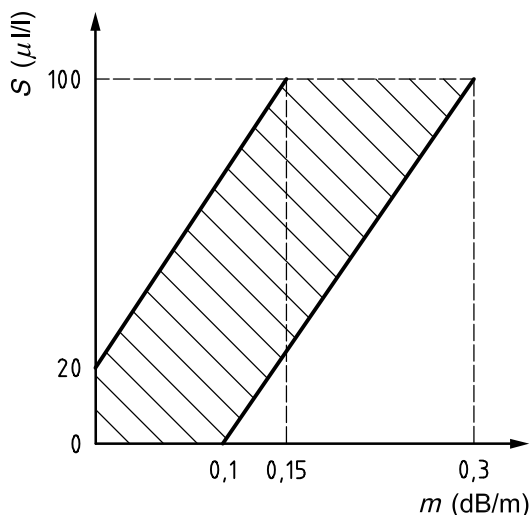
Figure 29 — Limits for S against m , Fire TF9
