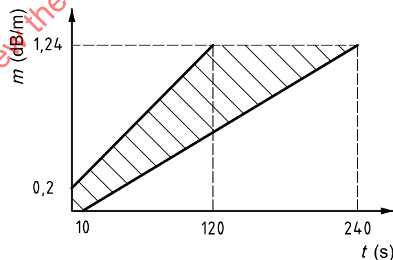
Figure 19 — Limits for m against time, t , Fire TF5
