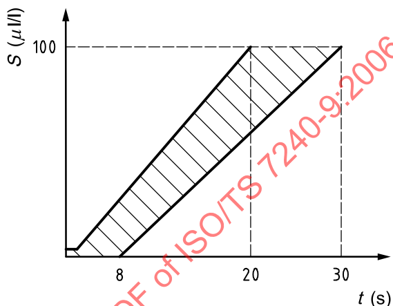
Figure 30 — Limits for S against time, t , Fire TF9
