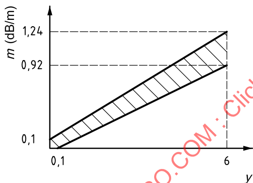
Figure 18 — Limits for m against y , Fire TF5
