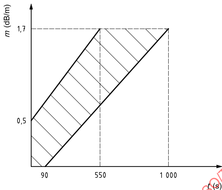
Figure 26 — Limits for m against time, t , Fire TF8
