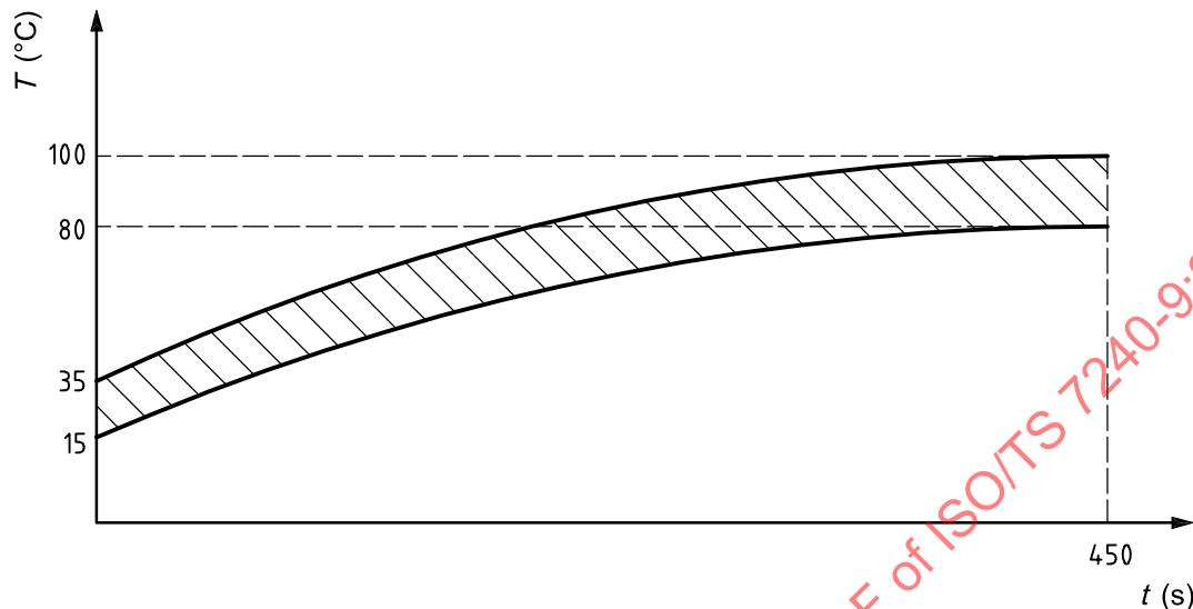
Figure 21 — Limits for T against t , Fire TF6
