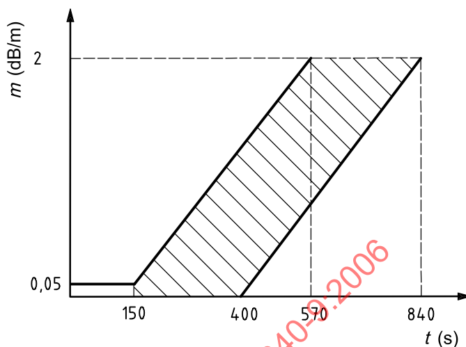
Figure 9 — Limits for m against time, t , Fire TF2
