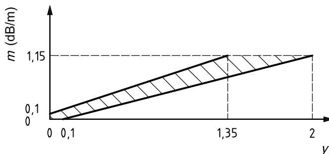
Figure 23 — Limits for m against y , Fire TF7
