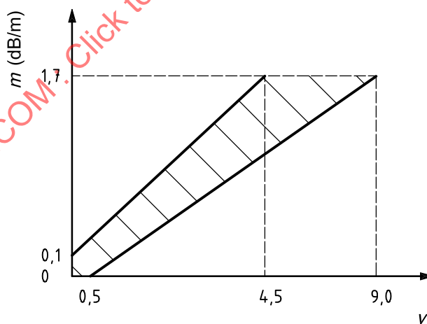
Figure 25 — Limits for m against y , Fire TF8
