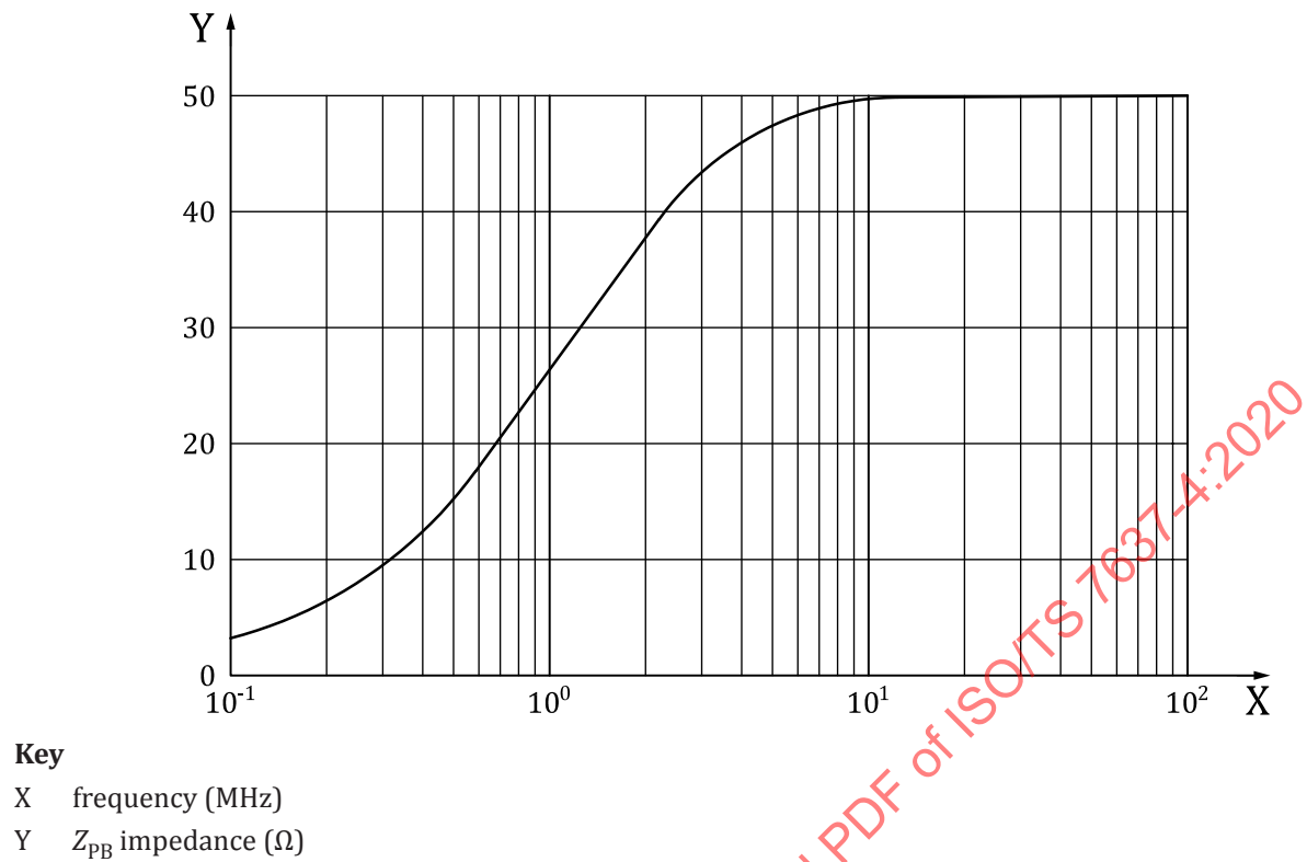
Figure 9 — Characteristic impedance of the HV-AN
