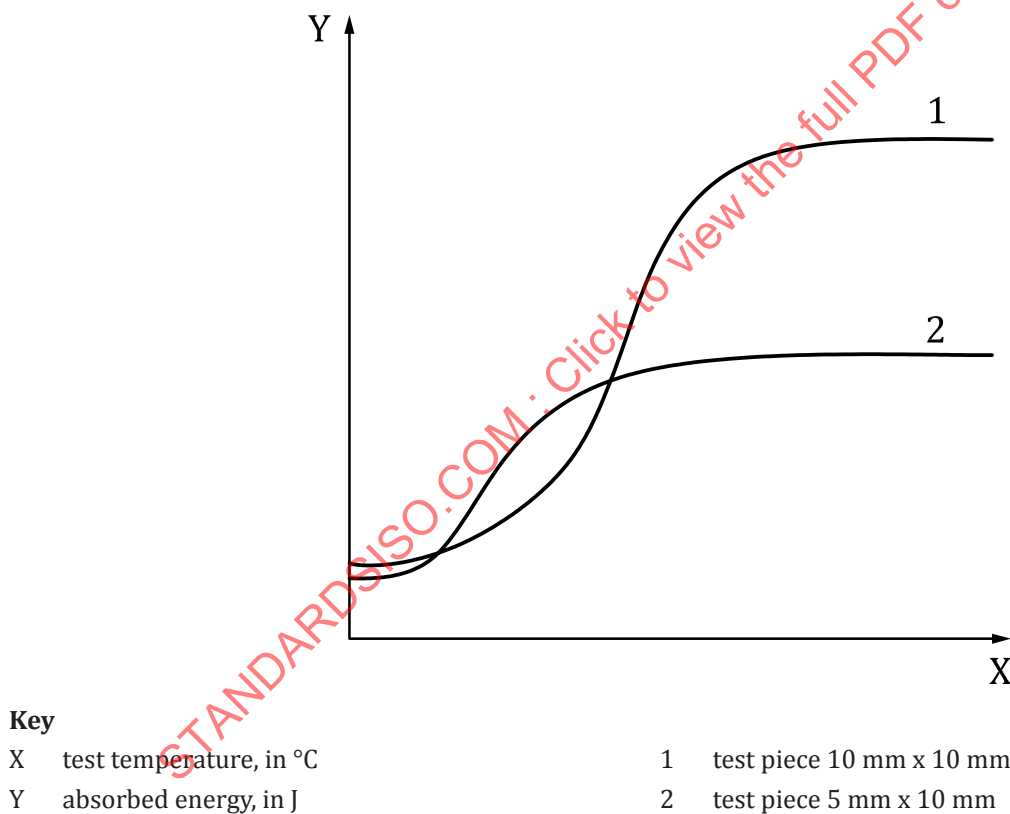
Figure 3 — Example of an impact test curve for a material with subsize test pieces
