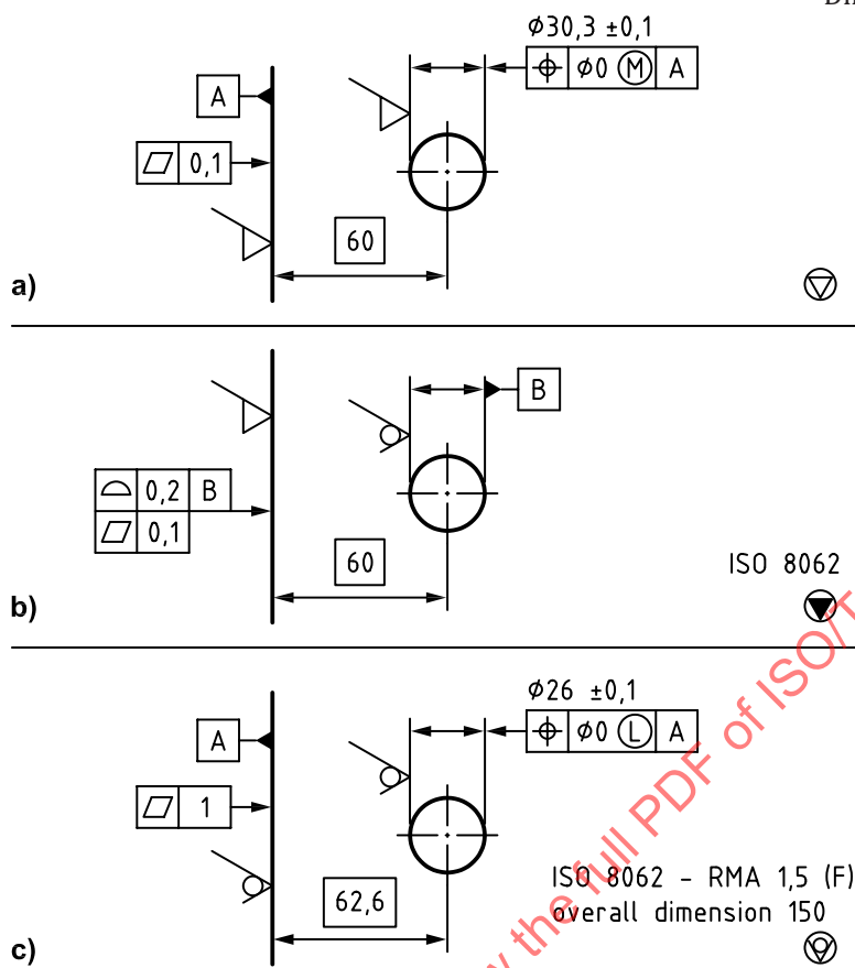
Figure D.1 — Feature of size (hole) relative to a plane datum, requirements
