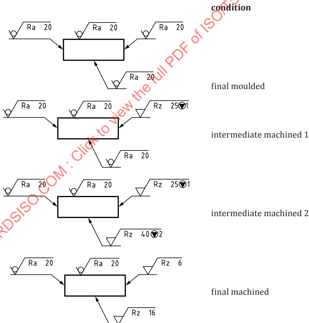
Figure 8 — Example of a surface texture indication on a combined drawing and its interpretation
