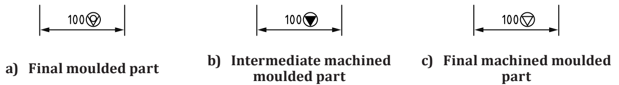
Figure 9 — Examples of nominal dimensions
