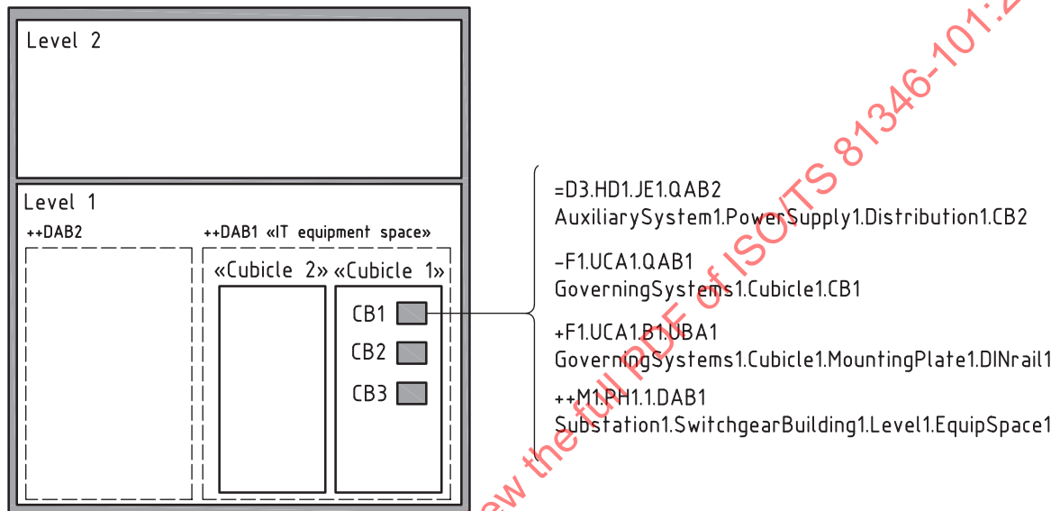
Figure A.1 — RD-set of a circuit breaker
