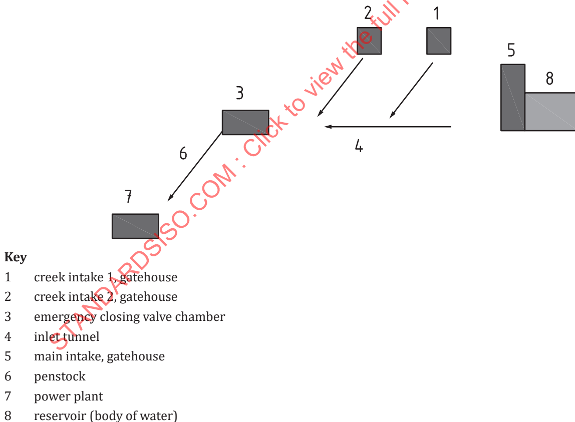
Figure 40 — Example of a water transport system in a hydropower plant — Construction works point of view
