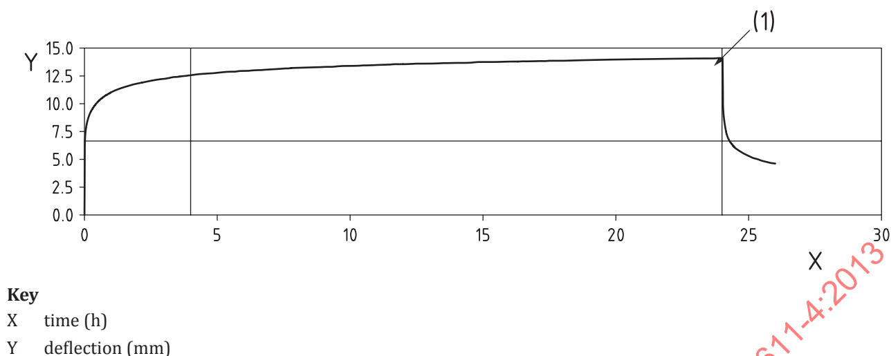
Figure A.1 — Actual deflection curve measurement
