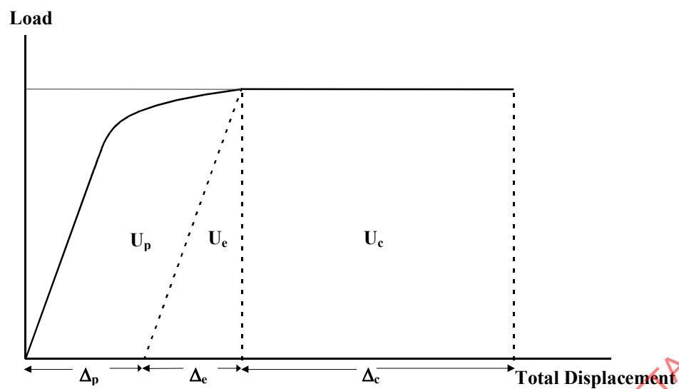
Figure A.II.7: Schematic Load-Displacement Behaviour from a Constant Load Creep Crack Growth Test
