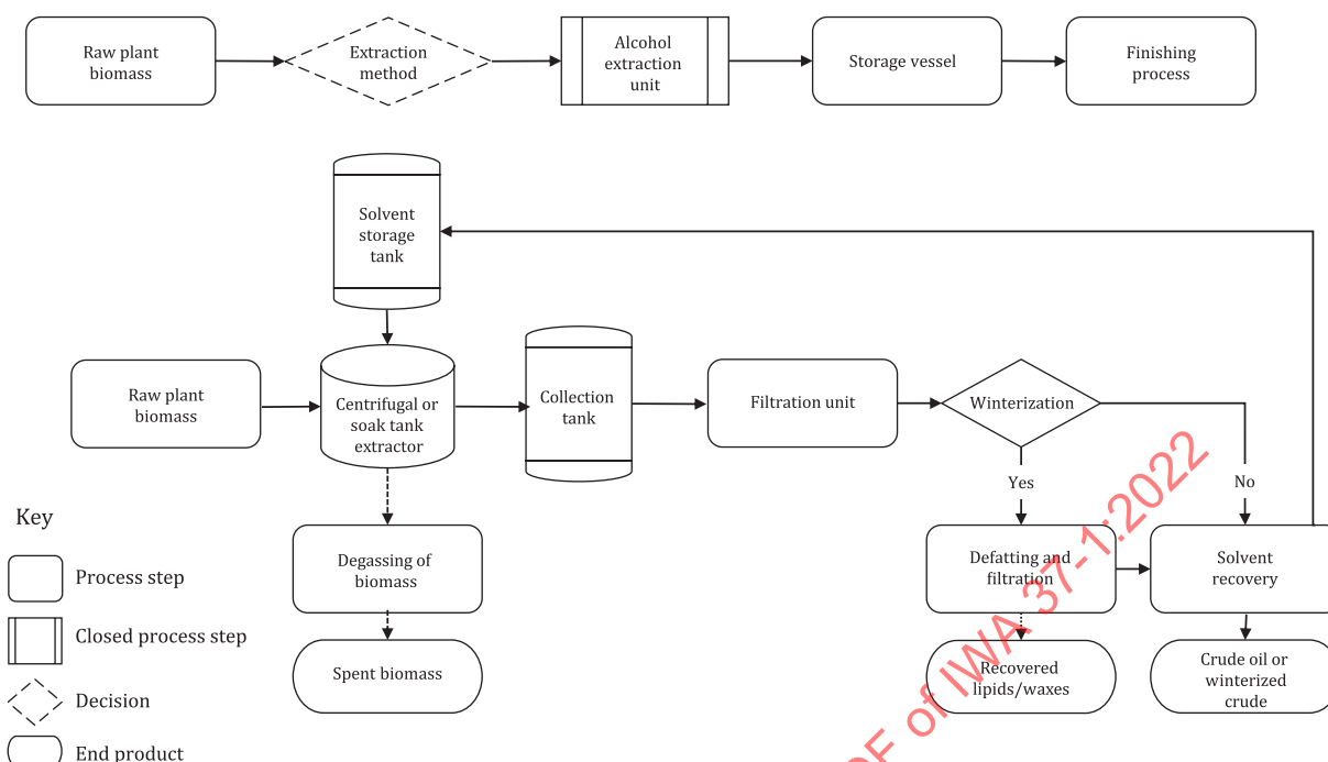
Figure 4 — Alcohol extraction process flow
