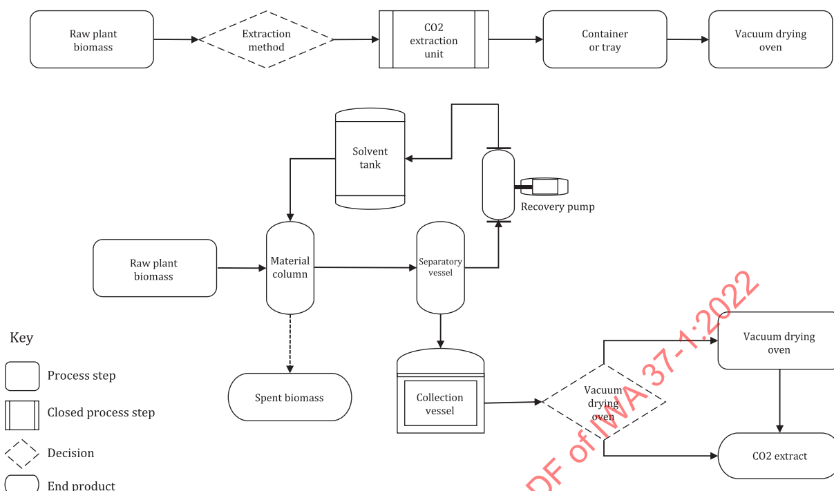
Figure 3 — Carbon dioxide extraction process flow
