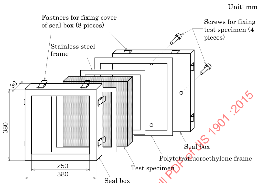
Figure JC.2 The composition of seal box (example)
