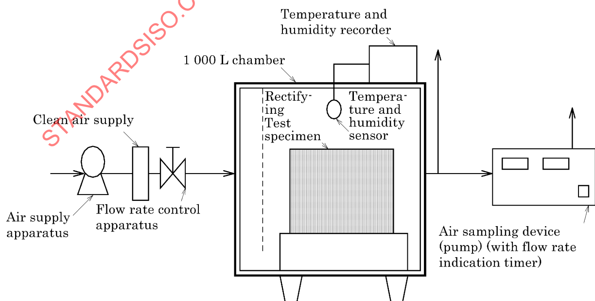
Figure JC 1 Composition of 1 000 L chamber system
