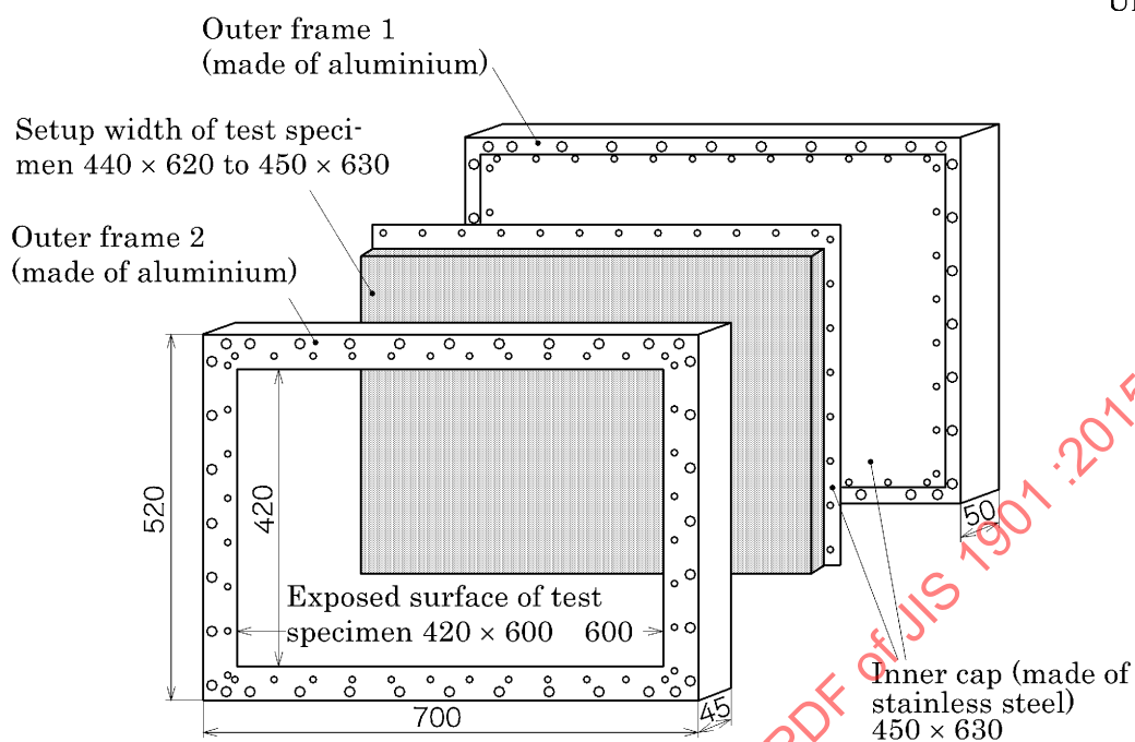
Figure JB.3 The composition of seal box (example)
