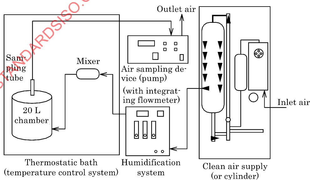
Figure JA.1 Composition of 20 L chamber system
