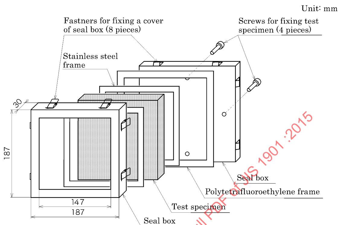
Figure JA.3 The composition of seal box (example)
