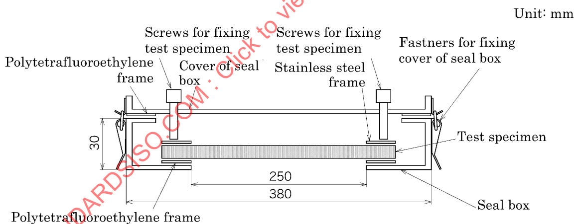
Figure JC.3 The cross-section of seal box (example)
