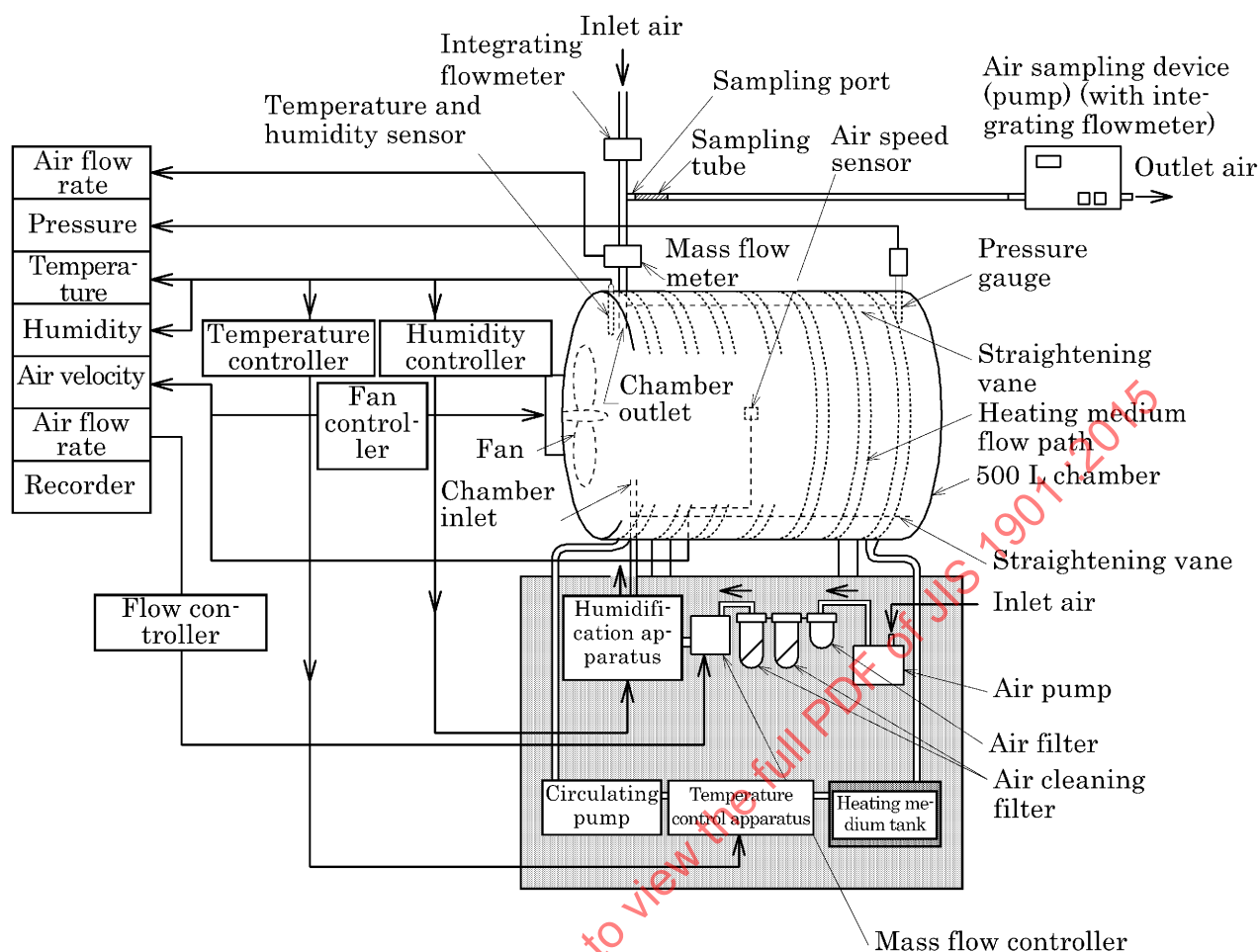
Figure JB.1 Composition of 500 L chamber system
