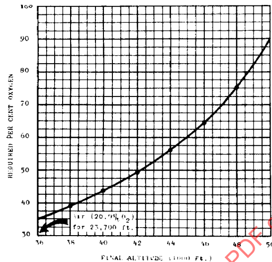
FIGURE 3 - Breathing Mixtures Before Decompression
