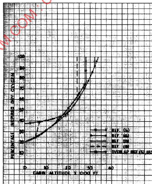
FIGURE 2 - Comparison of Oxygen Concentration vs. Altitude
