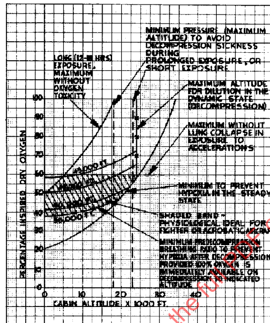
FIGURE 1 - Recommended Oxygen Concentration vs. Altitude
