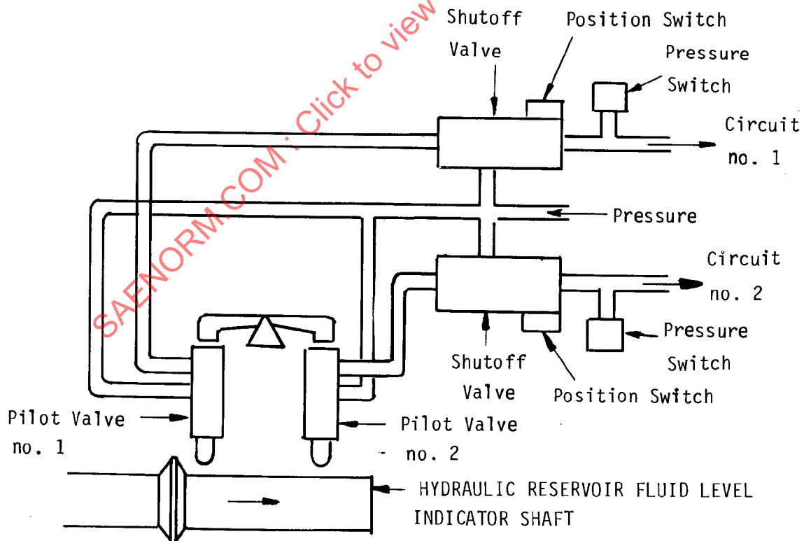
FIGURE 5. RESERVOIR FLUID LEVEL SENSING
