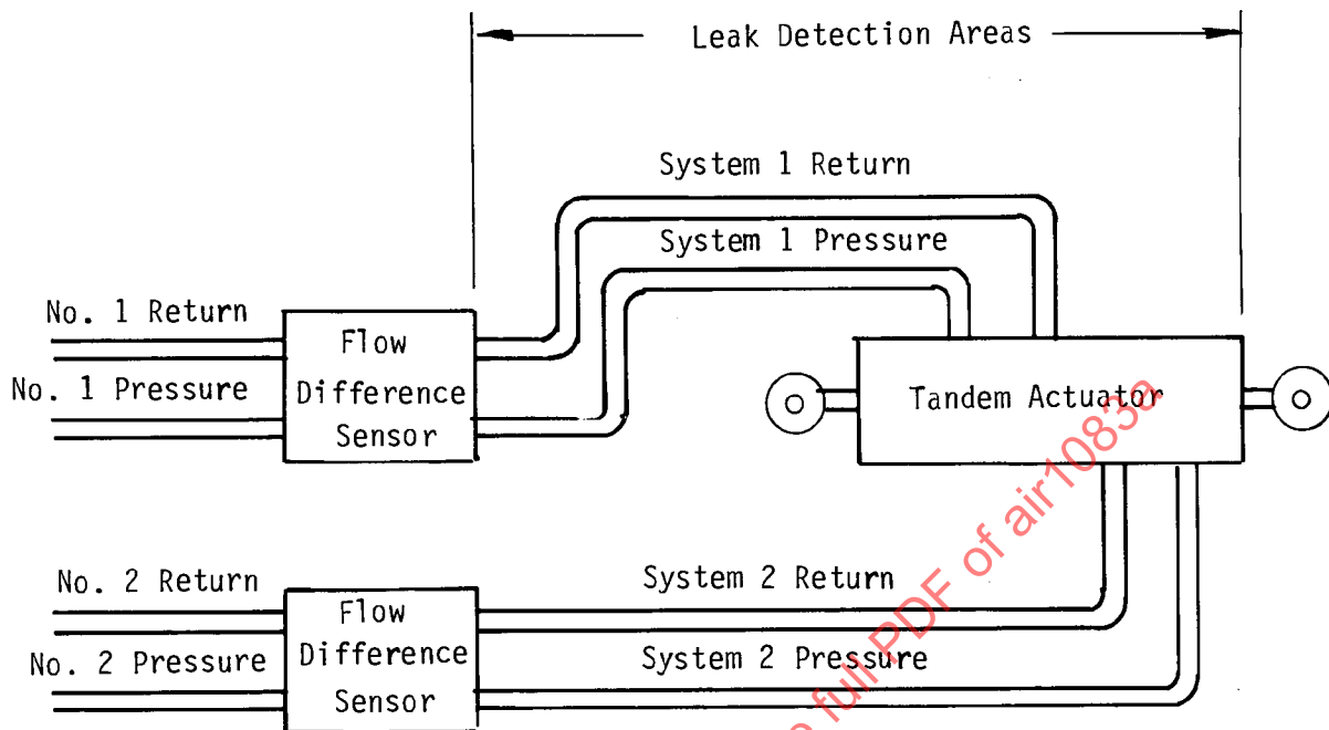
FIGURE 6. FLOW-DIFFERENCE-SENSING VALVE CIRCUIT
