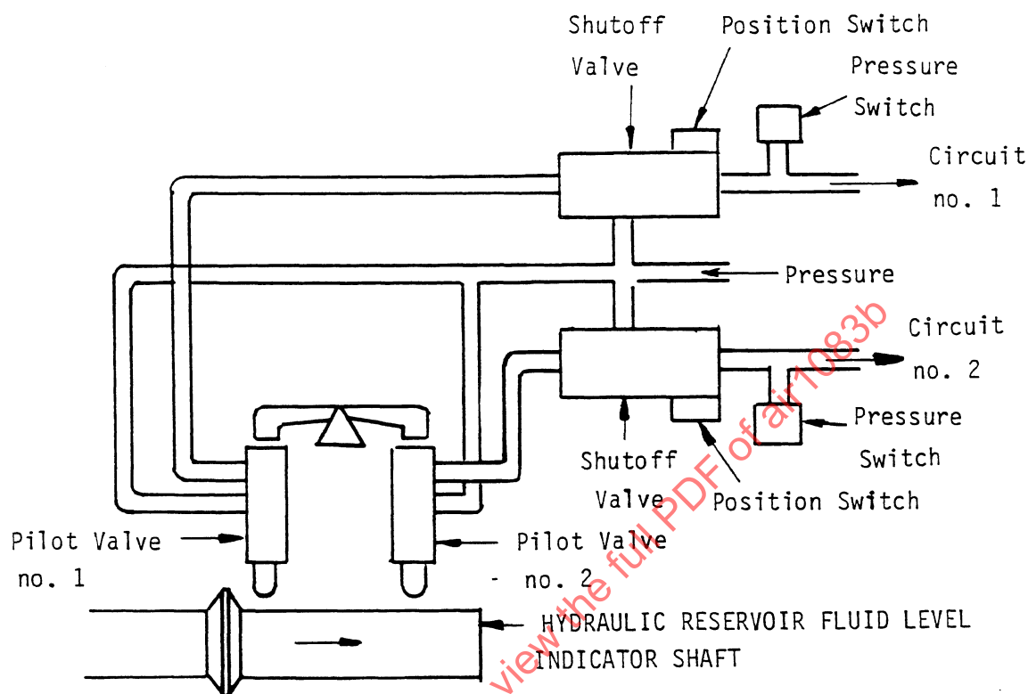
FIGURE 5 - Reservoir Level Sensing
