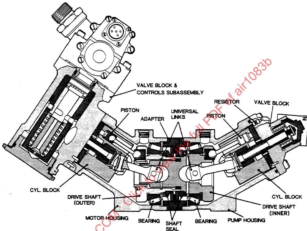
FIGURE 7 - Power Transfer Unit (PTU)
