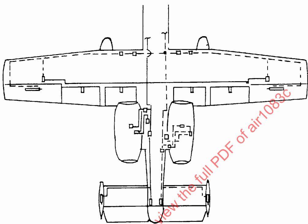
FIGURE 3 - A-10 SKETCH (EXAMPLE) SHOWING PHYSICAL SEPARATION OF HYDRAULIC CIRCUITS
