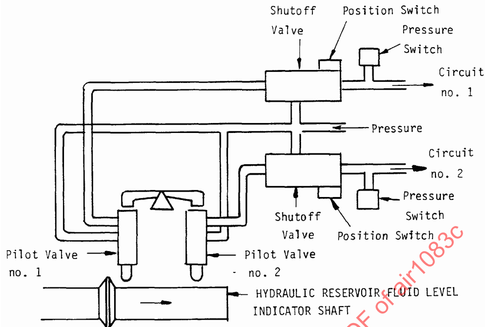
FIGURE 5 - RESERVOIR LEVEL SENSING
