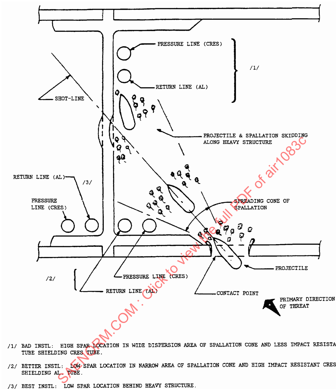
FIGURE 4 - ENHANCEMENT TECHNIQUES AGAINST SPALLATION THREAT
