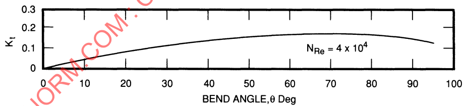
Figure 1A-35 - Loss Coefficient for Thin Noncircular Arc Vanes (From Ref. 1)
