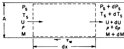
Figure 1B-18 - Control Volume
