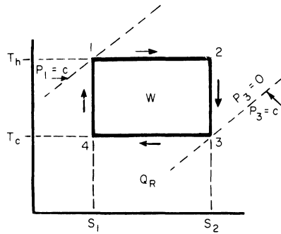
Figure 1B-3 - T-S Diagram
