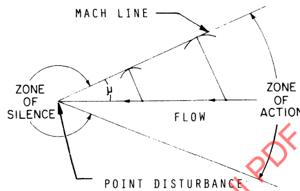
Figure 1B-21 - Mach Wave Formation
