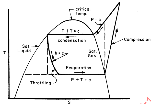
Figure 1B-6 - Rankine Vapor Cycle in Refrigeration
