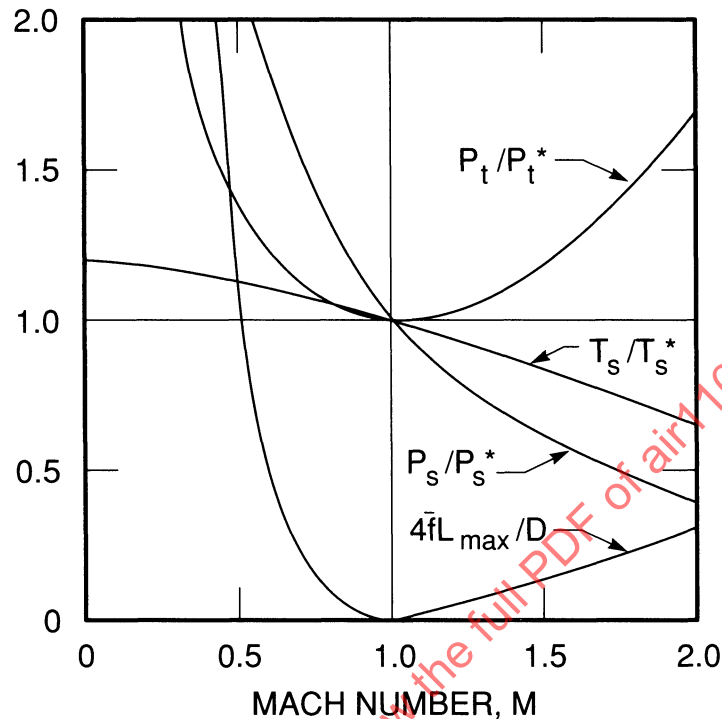
Figure 1B-20 - Effect of Wall Friction on Duct Flow Properties (The asterisk denotes integration of differential forms of flow property equations.)
