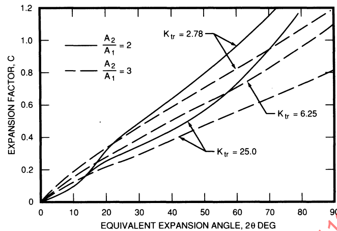
Figure 1A-51 - Expansion Factor for a Diffuser Followed by a Resistance Unit (From Ref. 26)
