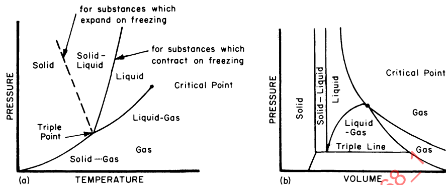
Figure 1B-9 - Solid and Liquid Phases with Changing P , V , T
