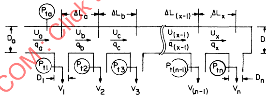
Figure 1A-59 - Sketch of a Typical Manifold
