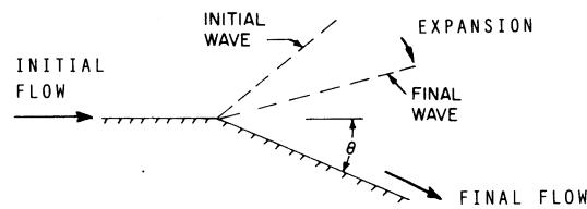
Figure 1B-23 - Expansion Fan
