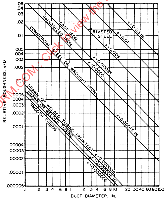
Figure 1A-4 - Relative Roughness, Circular Ducts
