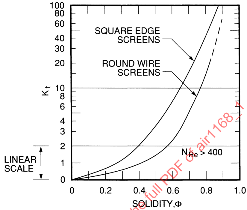
Figure 1A-62 - Loss Coefficients for Screens and Grids (From Ref. 56)
