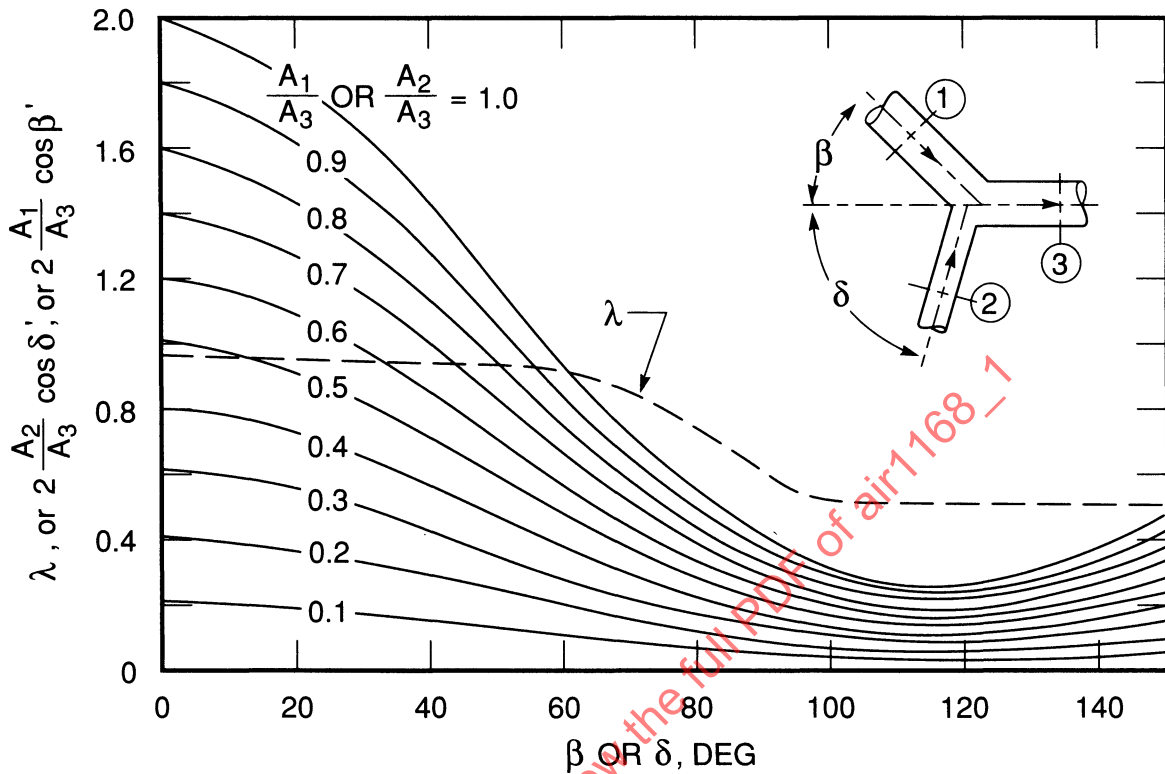
Figure 1A-58 - Converging Branch, Functions for Computing Loss Coefficient (From Ref. 7)
