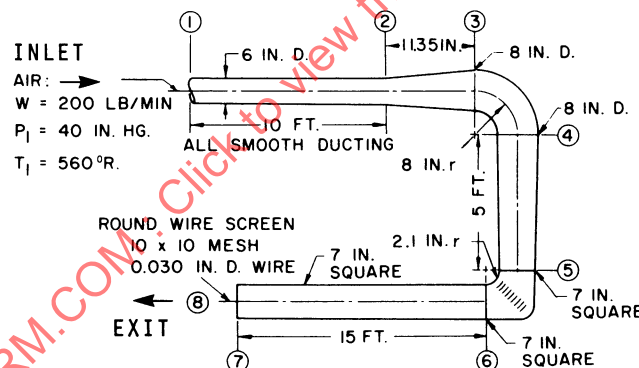
Figure 1A-65 - Example of a Duct System for Flow Loss Calculations
