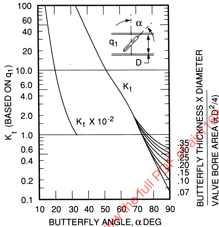
Figure 1A-61 - Loss Coefficient, Butterfly Valves (From Ref. 65)
