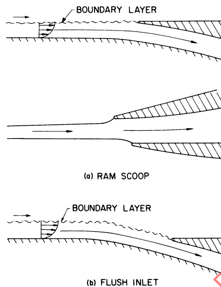
Figure 1B-29 - Types and Locations of Auxiliary Inlets. (a) Ram Scoop; (b) Flush Inlet
