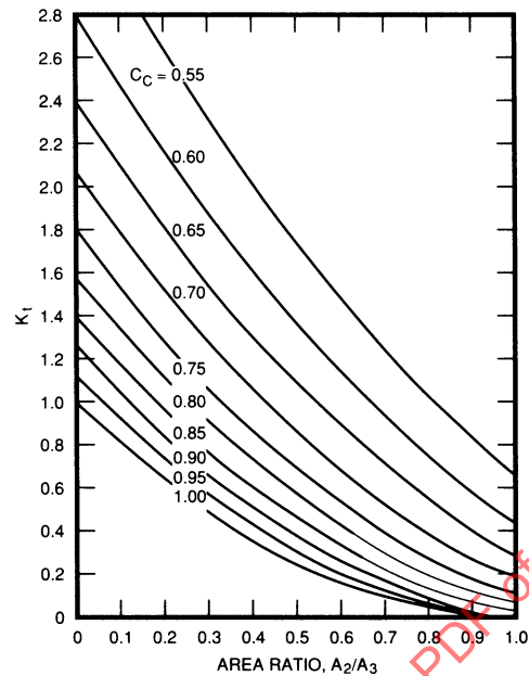
Figure 1A-54 - Loss Coefficient for an Orifice in a Duct: K_1 = [(1/C_c) - (A_2/A_3)]^2
