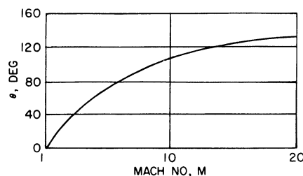
Figure 1B-24 - Prandtl-Meyer Function
