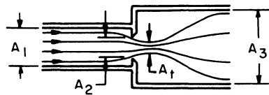
Figure 1A-52 - Sketch of an Orifice in a Duct
