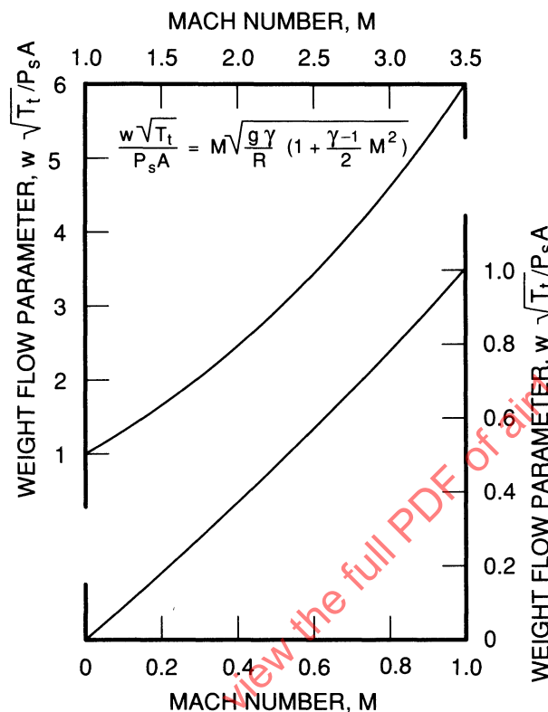
Figure 1B-13 - Weight Flow Parameter, w\sqrt{T_t}/P_s A , as a Function of Mach Number
