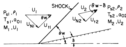
Figure 1B-26 - Oblique Shock Diagram
