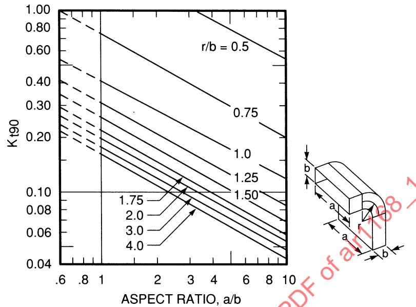
Figure 1A-18 - Loss Coefficient for 90 deg Bends, Rectangular Ducts, N_{Re} = 100,000 (From Ref. 1, Fig. 2a)
