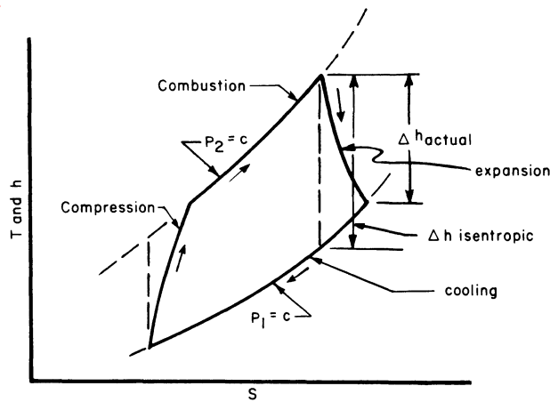
Figure 1B-5 - Brayton Cycle
