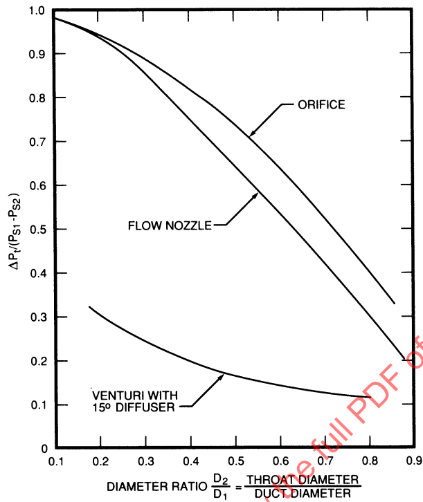
Figure 1A-56 - Approximate Pressure Loss Through Several ASME Flow Metering Devices P_{s1} = Upstream Static Pressure; P_{s2} = Throat Static Pressure (From Ref. 35, Fig. 5)
