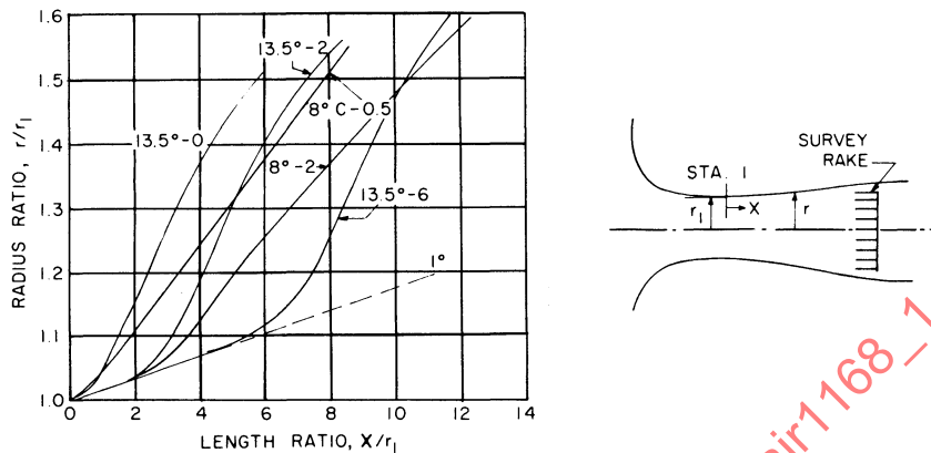
Figure 1B-27 - Geometric Properties of Diffusers Reported in Ref. 14 ( A_1/A_2 = 0.510 rake station; r_1 = 1.50 in. Diffuser identification system: (1) first number refers to maximum total divergence angle, (2) second number refers to throat extension in terms of inlet throat radii, (3) letter C refers to conical diffuser).
