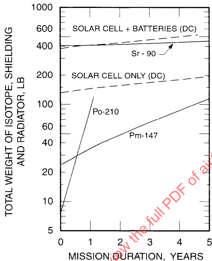
Figure 14-18 - Weight penalty comparison; 1 kW system
