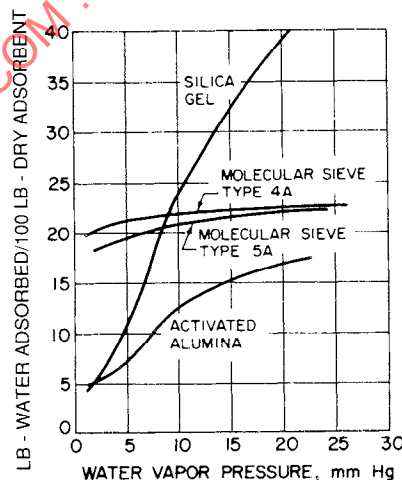
Figure 14-19 - Water adsorption isotherms at 77°F
