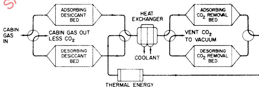
Figure 14-32 - Purge gas desorbed desiccant
