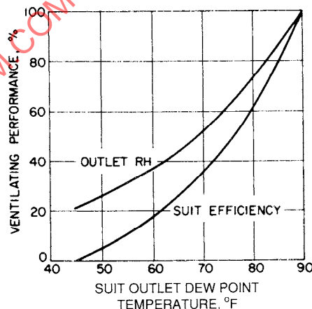
Figure 14-11 - Suit efficiency and outlet gas relative humidity versus outlet dewpoint for 45°F saturated inlet gas and 90°F outlet dry bulb temperature; suit pressure = 3.5 psia O_2
