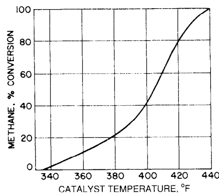
Figure 14-37 - Catalytic burner performance
