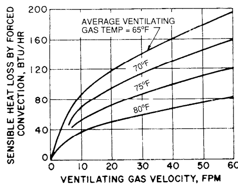
Figure 14-9 - Estimated convective heat loss from body; average t_{sk} = 91^\circ\text{F} , P_{amb} = 7.35 psia
