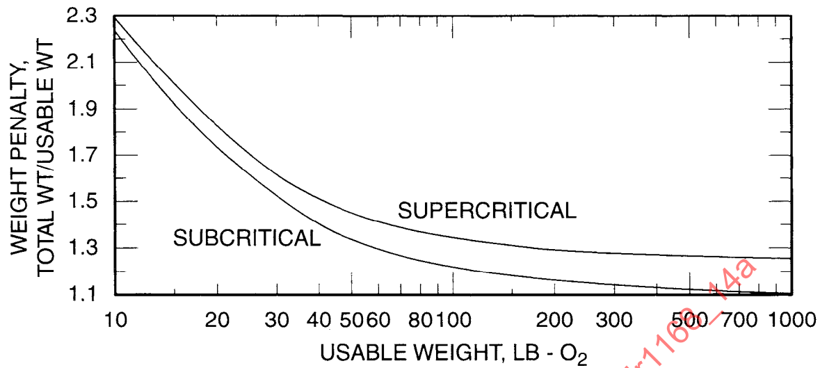
Figure 14-48 - Cryogenic oxygen tank weights as a function of usable weight. Conditions: P_c = 738 psia, 72 hr standby time, 1.0 lb / hr average flow rate, relief pressure = 1000 psia
