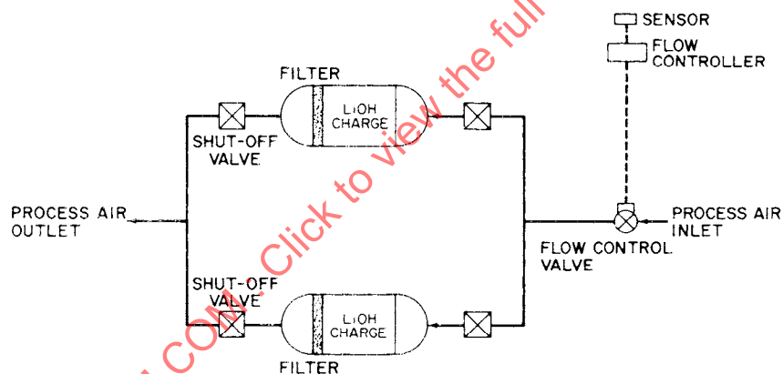
Figure 14-31 - Lithium hydroxide subsystem schematic diagram
