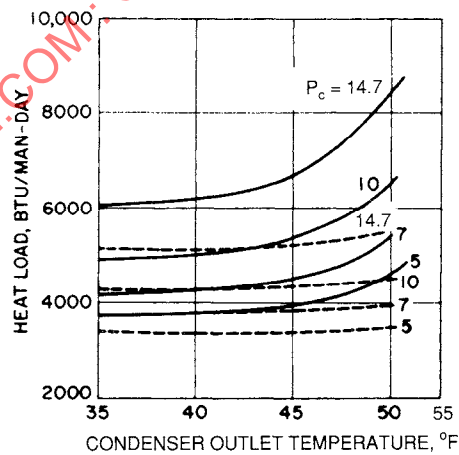
Figure 14-25 - Heat load variation with temperature; dotted curves at 70% RH, solid curves at 60% RH
