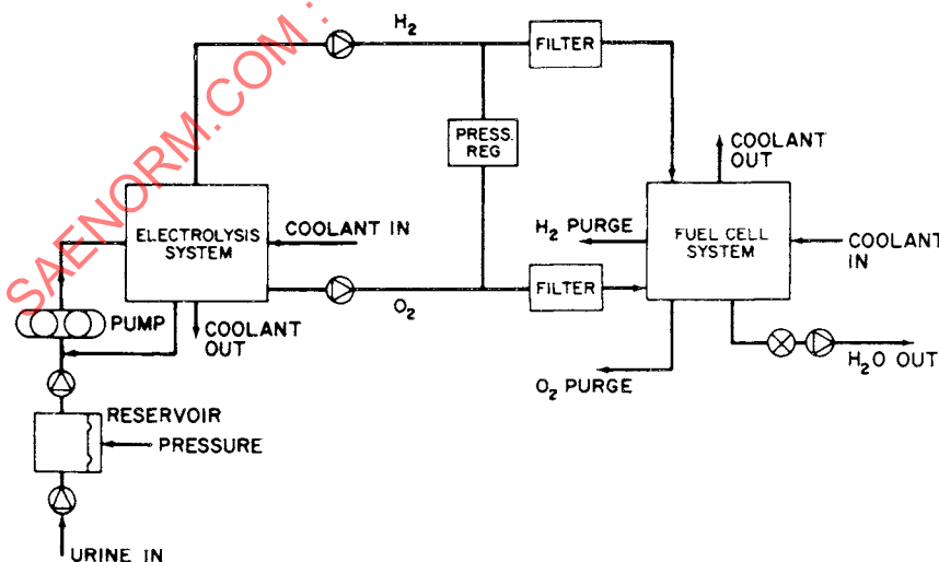
Figure 14-54 - Water reclamation by the ELF technique
