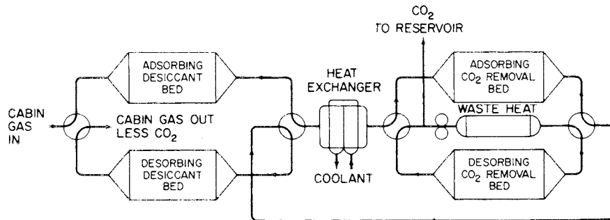
Figure 14-35 - Thermal desorbed CO 2 adsorbent
