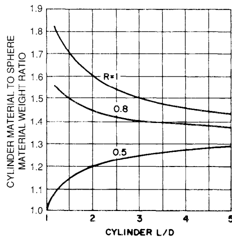
Figure 14-42 - Comparison of spherical and cylindrical vessel weights (L/D = overall length-to-diameter ratio)
