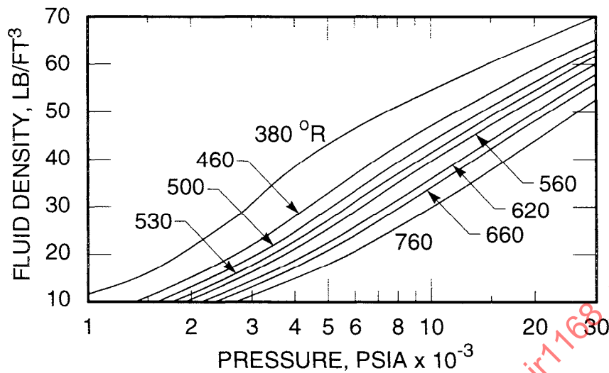
Figure 14-40 - Oxygen densities at high pressure
