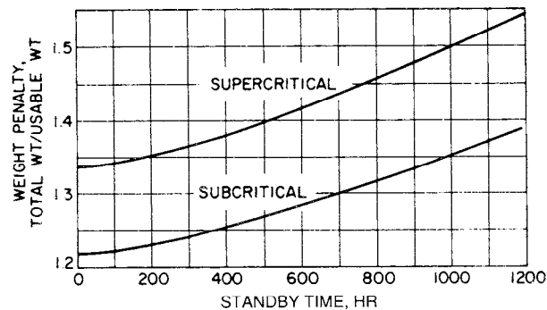
Figure 14-50 - Effect of nonvented standby time on cryogenic oxygen tank weights
