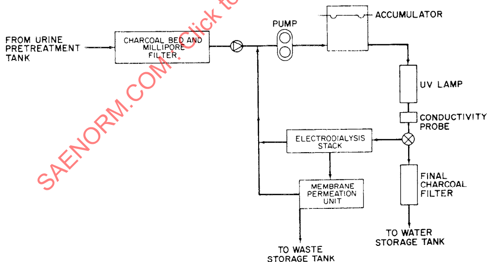
Figure 14-52 - Water reclamation by electrodialysis
