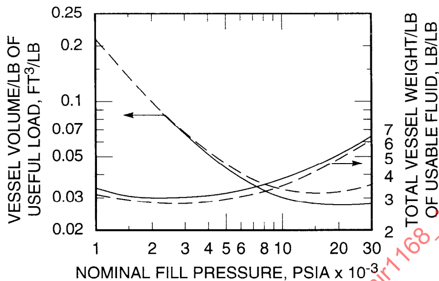
Figure 14-38 - Weight and volume of spherical oxygen storage vessels, safety factor 1.88; solid curves for SAE 4340 steel and dotted curves for Ti C-120 AV
