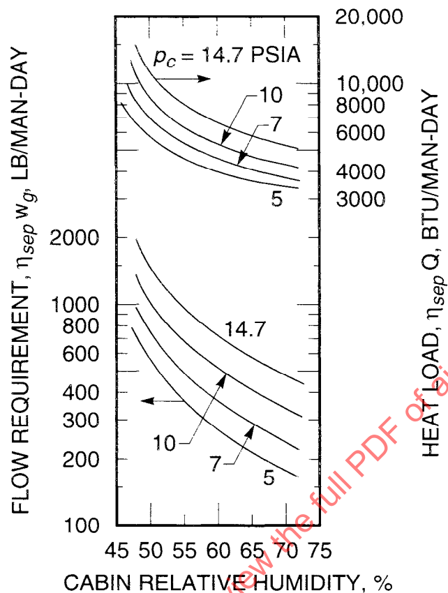
Figure 14-23 - Flow requirement and heat load for humidity control; condenser temperature 45°F
