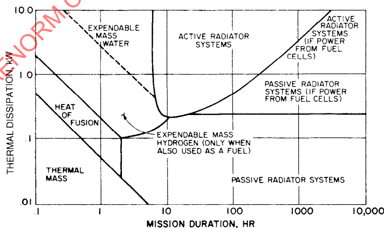
Figure 14-13 - Heat sink selection (summary)
