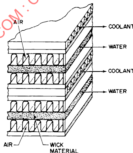
Figure 14-26 - A condenser/wick water separator fabrication method
