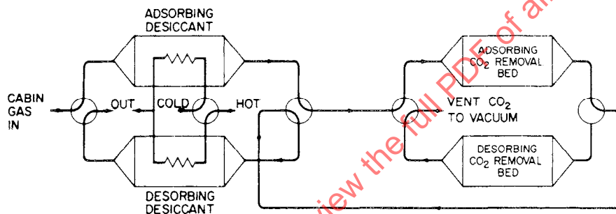
Figure 14-34 - Thermal swing desiccant desorption
