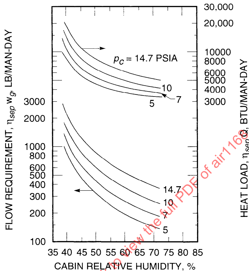
Figure 14-22 - Flow requirement and heat load for humidity control; condenser temperature 40°F
