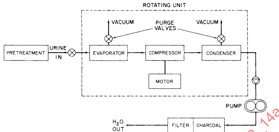
Figure 14-55 - Water reclamation by vapor compression
