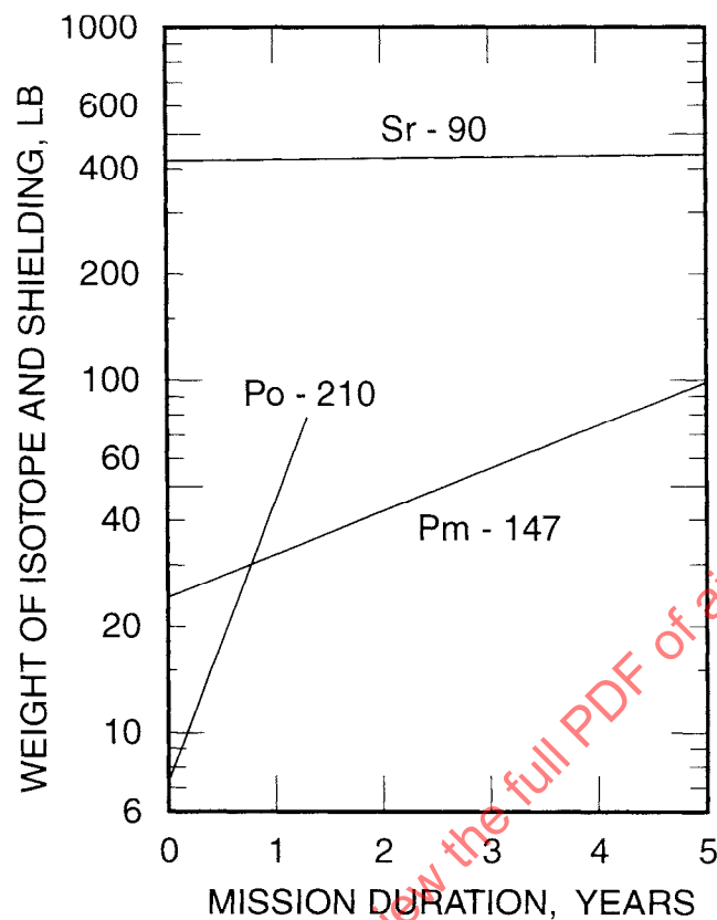
Figure 14-17 - Shielded isotope weights; 1 kW system, shielding U-238, dose rate = 20 mrem / hr at 3 ft
