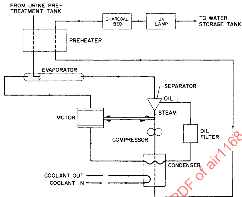
Figure 14-56 - Water reclamation by oil jet evaporation
