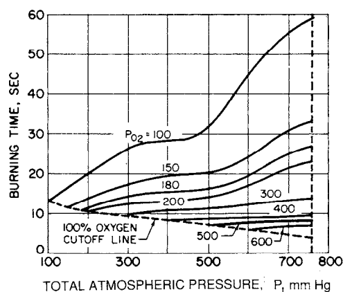
Figure 14-6 - Effect of oxygen partial pressure on burning time; P_{O_2} in mm Hg; (Ref. 15)
