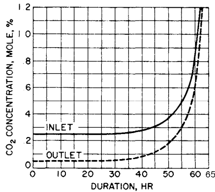
Figure 14-28 - Typical closed circuit LiOH performance; pellet size, 4-8 mesh; bed length, 8.0 in.; bed diameter, 6.0 in.; absorbent weight, 3.5 lb; air weight flow, 43 lb / hr; CO 2 weight flow, 0.043 lb / hr; air superficial velocity, 50 fpm; air total pressure, 14.7 psia; air inlet temperature, 182°F
