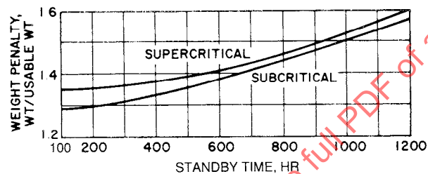
Figure 14-51 - Effect of nonvented standby time on cryogenic nitrogen tank weights
