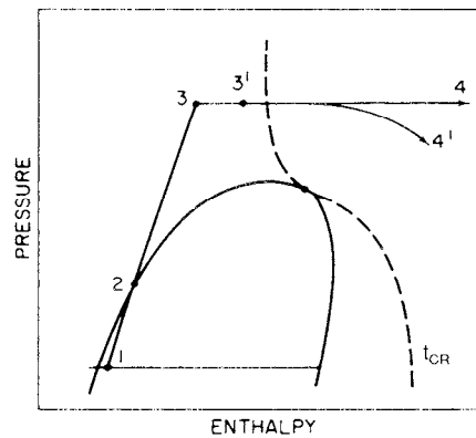
Figure 14-44 - Pressure-enthalpy diagram, thermally pressurized supercritical storage; points 1 = fill, 1-3 = initial pressurization, 3-3' = standby venting, 3-4 = constant pressure withdrawal
