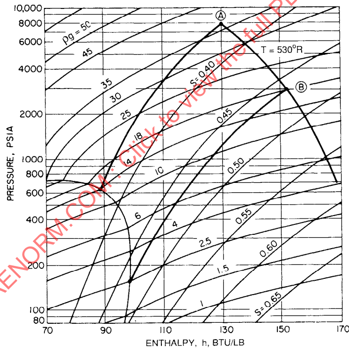
Figure 14-43 - Isentropic blowdown process; temperature, 530°R
