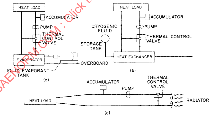
Figure 14-7 - Typical cooling systems; (a) expendable evaporant, (b) cryogenic fluid, (c) radiator
