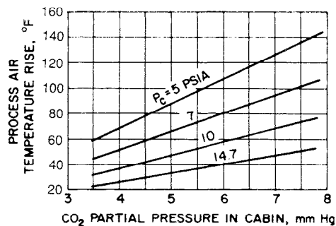
Figure 14-30 - Lithium hydroxide subsystem process air temperature rise
