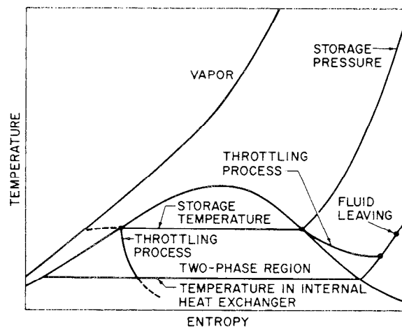
Figure 14-46 - Temperature-entropy diagram describing subcritical storage with vapor removal
