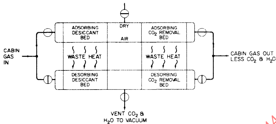
Figure 14-33 - Vacuum desorbed desiccant
