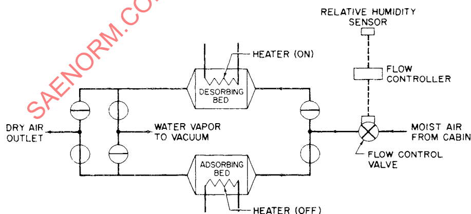
Figure 14-20 - Regenerable silica gel humidity control subsystem
