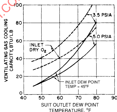
Figure 14-12 - Cooling capacity of suit ventilating gas, assuming 90°F outlet dry bulb temperature and 45°F inlet dry bulb temperature
