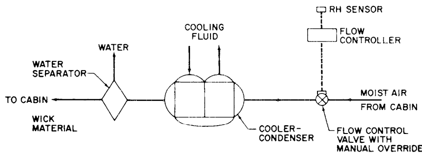
Figure 14-21 - Cooler-condenser humidity control subsystem
