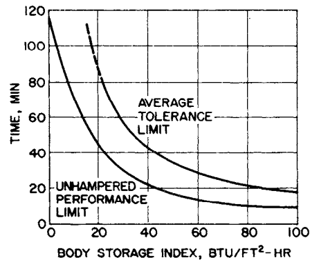
Figure 14-3 - Thermal tolerance limits (Ref. 23)
