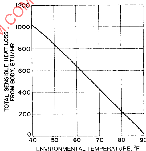
Figure 14-10 - Total sensible heat loss from body for shirtsleeve environment; t_{sk} = 91^{\circ}\text{F} , v_{gas} = 40 fpm
