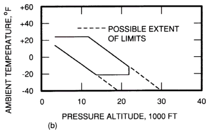
FIGURE 27 - Intermittent Maximum Icing Condition. Altitude: 4000 to 22,000 ft; horizontal extent: 2.6 nmi, (a) liquid water content, (b) envelope of icing temperature
