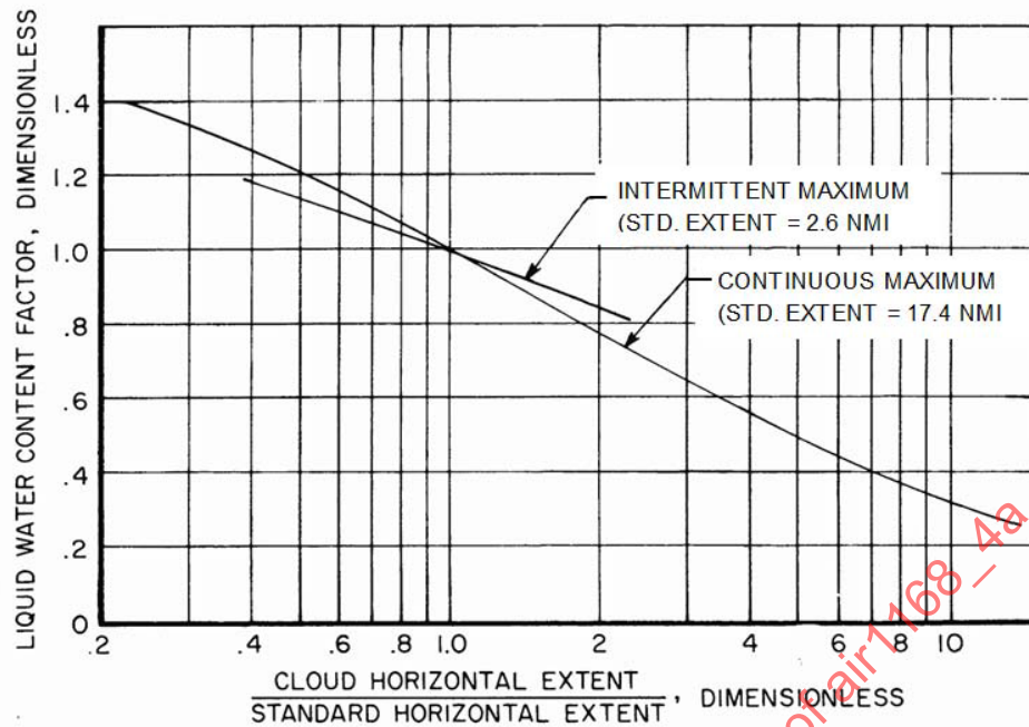
FIGURE 26 - Variation of Liquid Water Content with Cloud Horizontal Extent
