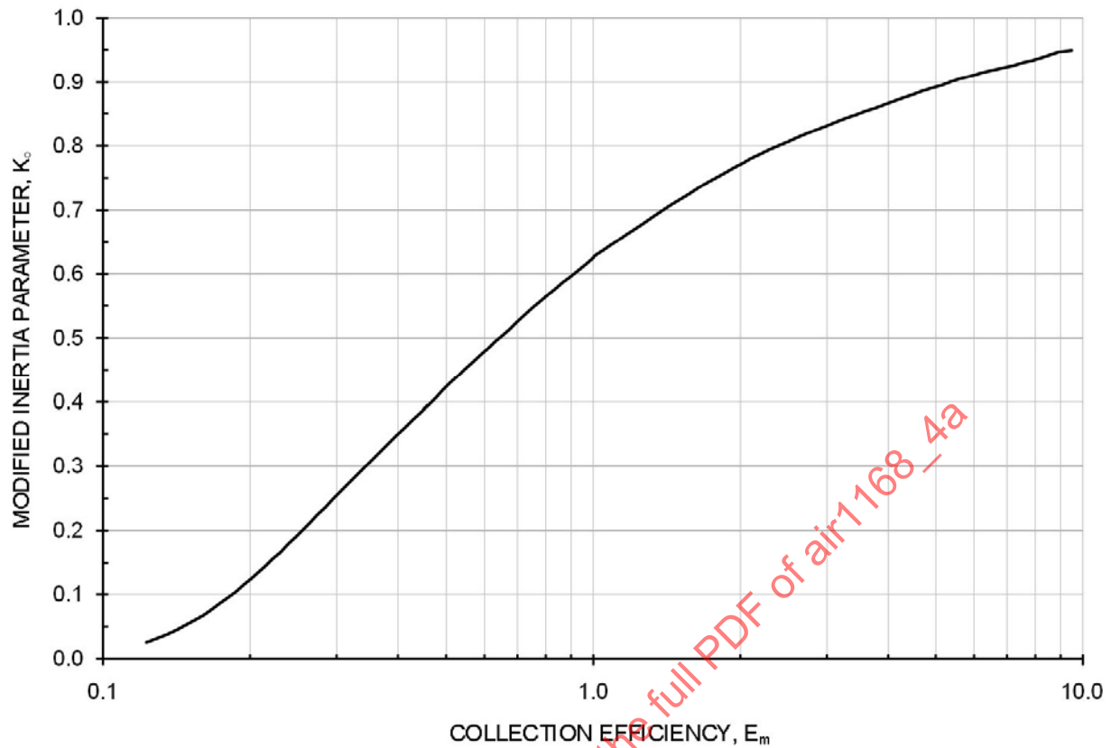
FIGURE 33 - Collection Efficiency of Windshields (Based on Semi-infinite Rectangle)
