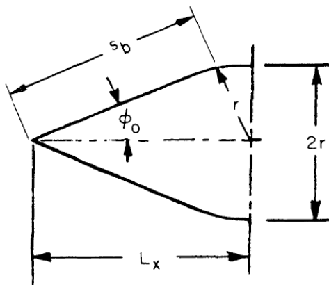
FIGURE 10 - Cone Geometry
