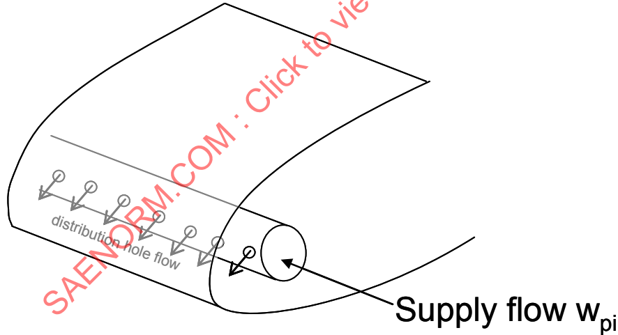
FIGURE 19 - Piccolo Tube in a Leading Edge
