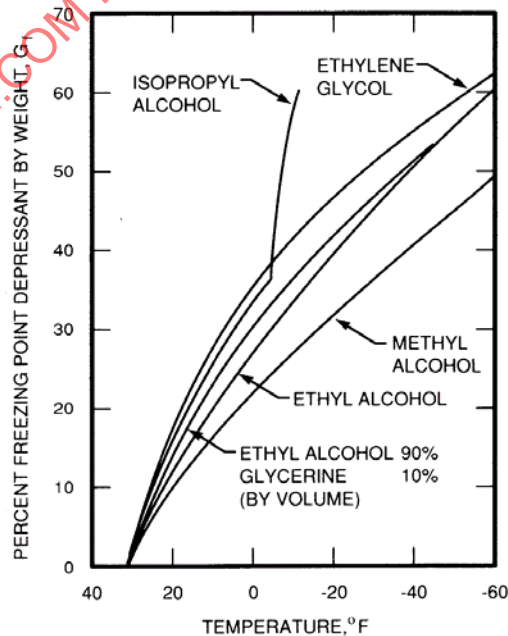
FIGURE 37 - Freezing Points for Aqueous Solutions of Several Fluids
