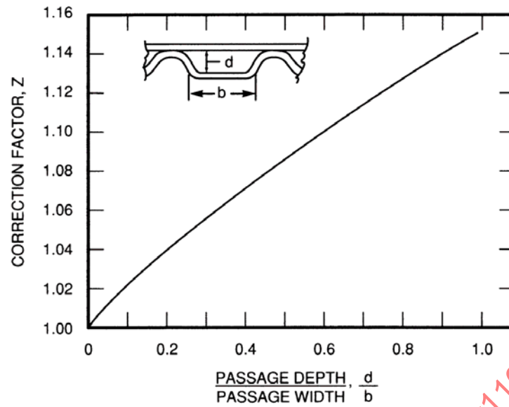
FIGURE 18 - Correction Factor for Passage Aspect Ratio, Z = (1+d/b)^{0.2}
