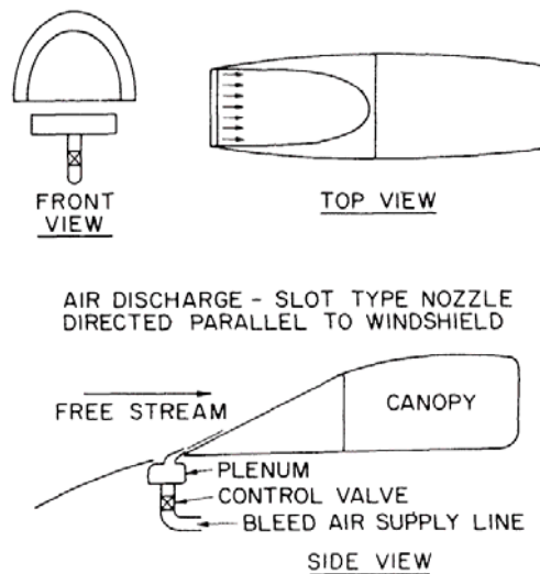
FIGURE 31 - External Air Blast Windshield Anti-icing and Rain Removal System
