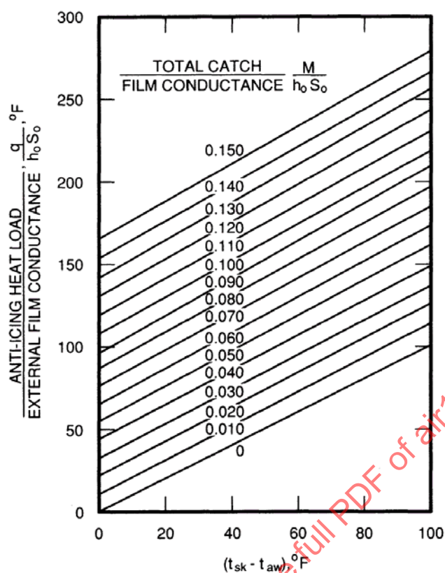
FIGURE 15 - Airfoil Evaporative Anti-icing Energy Requirements
