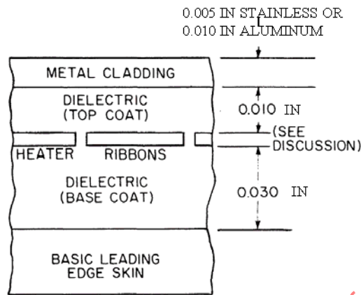
FIGURE 23 - Example Heater Construction
