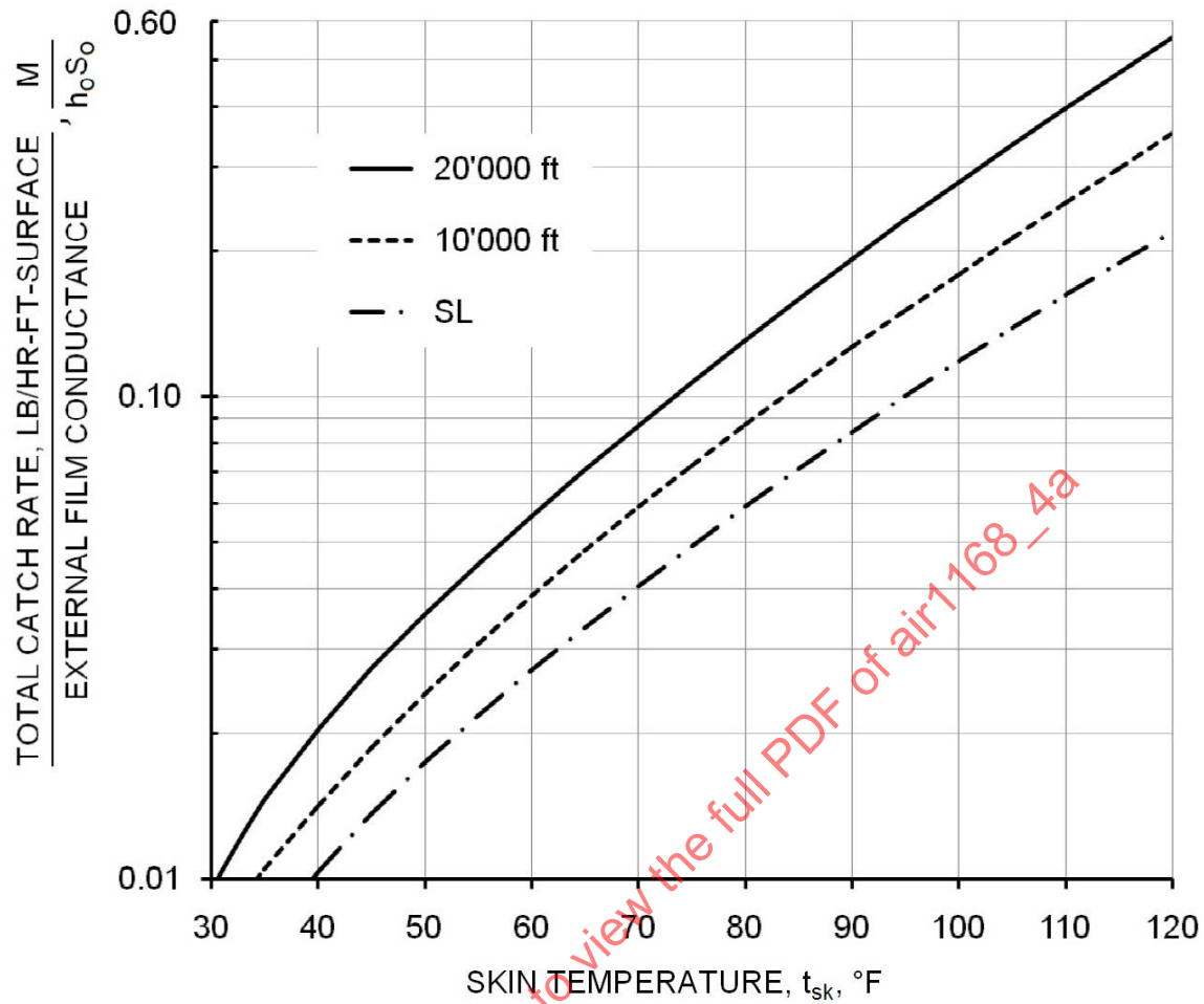
FIGURE 14 - Skin Temperature Required for Evaporative Anti-icing
