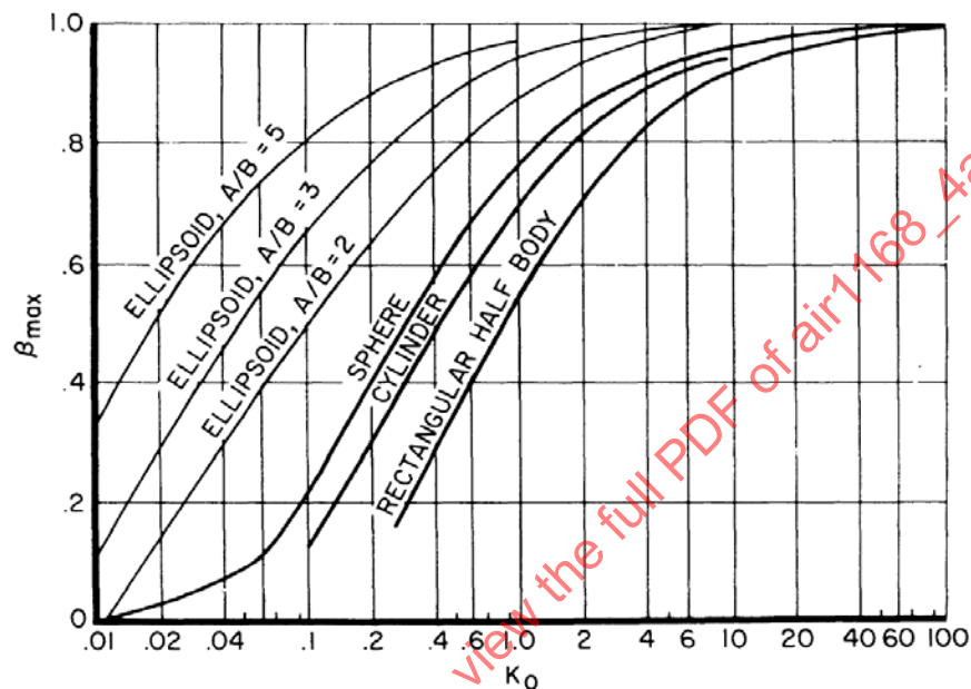
FIGURE 4 - Maximum Water Catch Efficiencies at the Stagnation Line, \alpha = 0 deg
