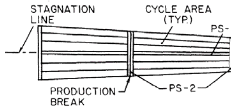
FIGURE 22 - Half Wing Heater Layout
