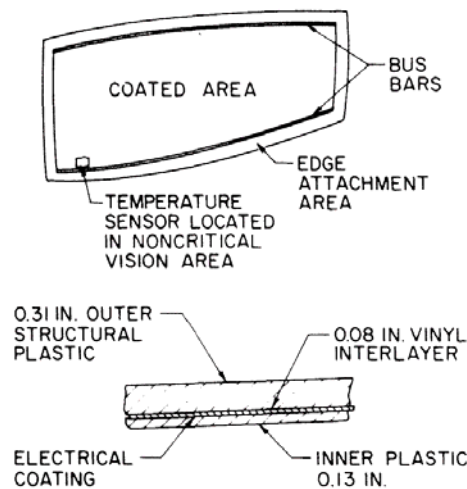
FIGURE 38 - Antifog Coating and Bus Bar Arrangement for Electrical Antifog on Plastic Canopy (or Windshield) Panel
