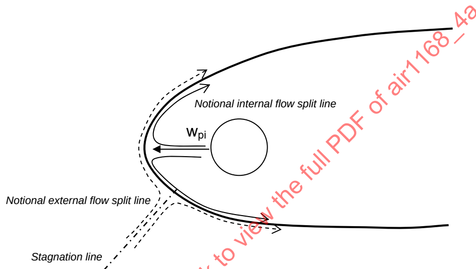
FIGURE 20 Flow Split on a Heated Airfoil Leading Edge
