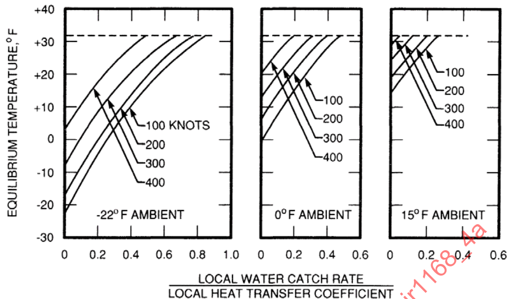
FIGURE 25 - Unheated Equilibrium Temperature of an Iced Surface, All Altitudes
