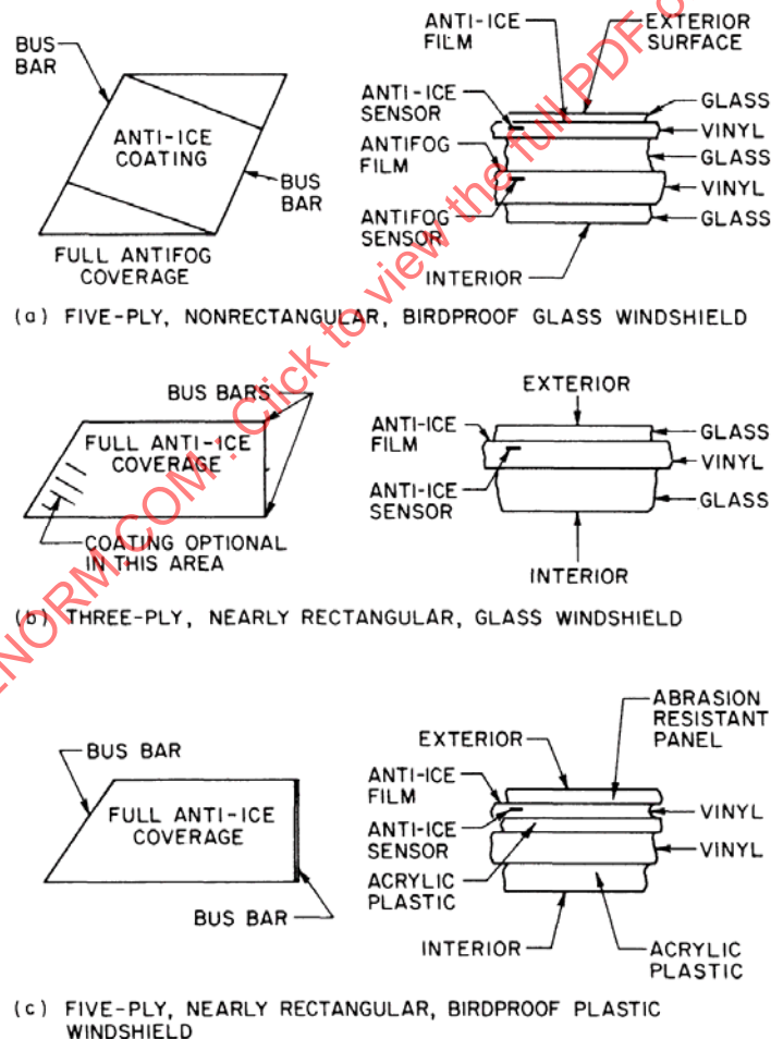
FIGURE 29 - Typical Windshield Panels Heated Electrically
