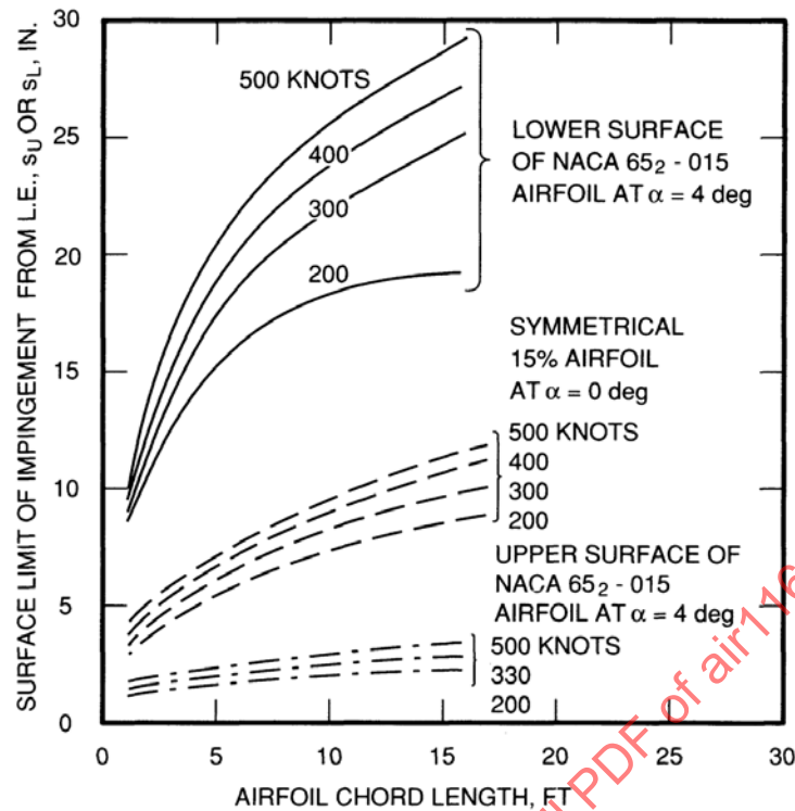
Figure 5 - Airfoil impingement limits for 40 \mu\text{m} maximum (20 \mu\text{m} volume median) drops (all altitudes: strictly true for a particular altitude and approximately, within 10%, true between sea level and 20000 feet)
