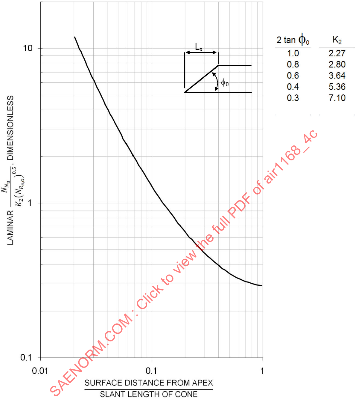
Figure 12 - Laminar heat transfer coefficients over cones
