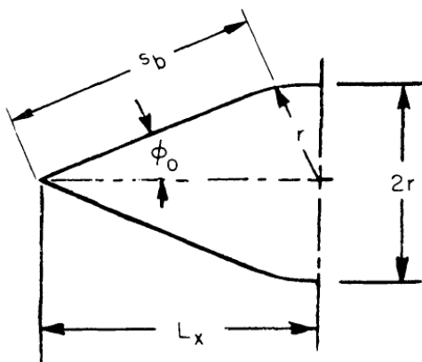
Figure 10 - Cone geometry
