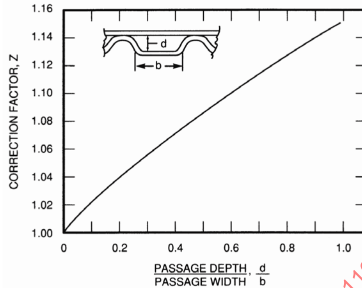
Figure 18 - Correction factor for passage aspect ratio; Z = (1+d/b)^{0.2}
