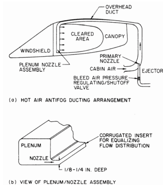
Figure 39 - Free jet air blast antifog or defog system using mixed compressor bleed and cabin air
