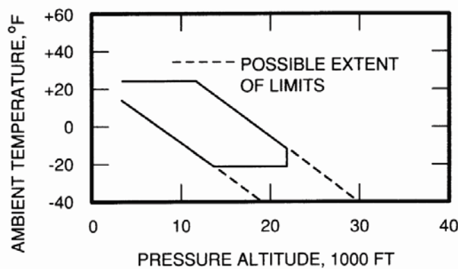
Figure 27 - Intermittent maximum icing condition. Altitude: 4000 to 22000 feet; horizontal extent: 2.6 nmi, (a) liquid water content, (b) envelope of icing temperature
