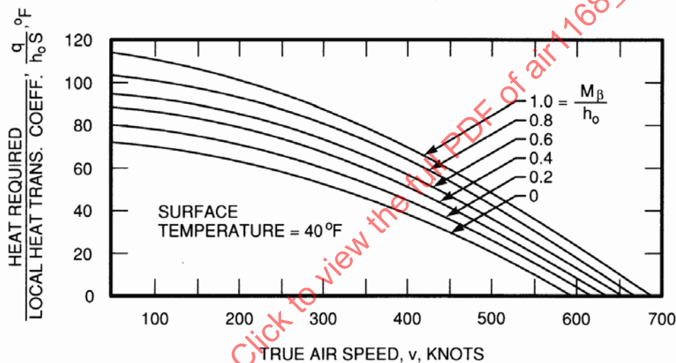
Figure 21 - Energy requirements for running wet anti-icing. Surface temperature = 40 °F, 10000 feet at 0 °F ambient. To obtain values for other altitudes: subtract 11.0 for sea level, add 15.0 for 22000 feet
