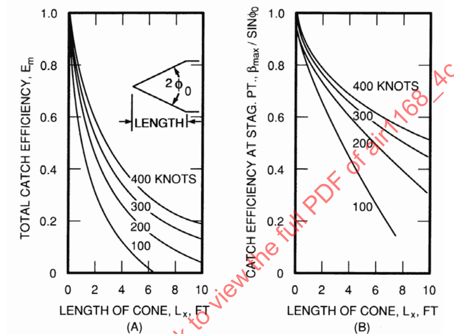
Figure 8 - Catch efficiency on cones for 20 \mu\text{m} volume median drops (A) - Total, (B) - Stagnation point (all altitudes: strictly true for 10000 feet altitude and approximately, within 10%, true between sea level and 20000 feet)
