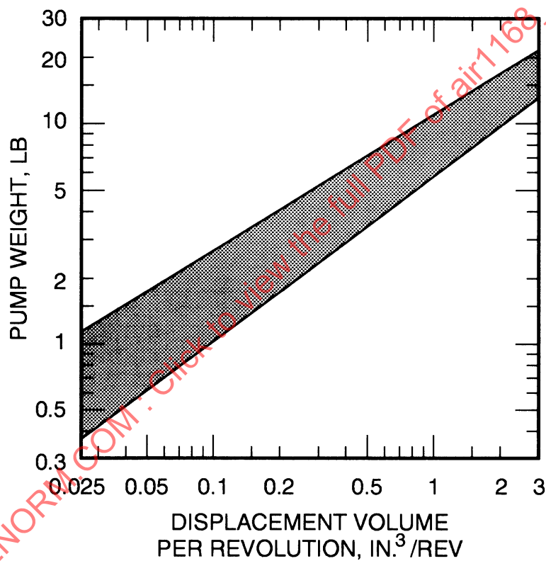
Figure 3H-15 - Approximate Weights for Piston, Gear, and Vane Pumps (Less Motor)
