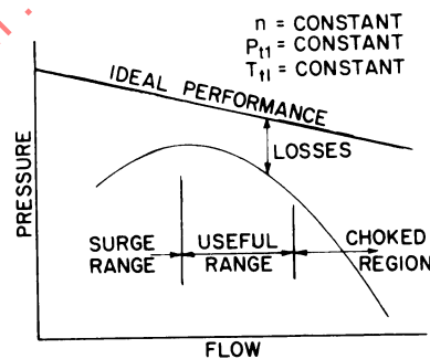
Figure 3H-37 - General Characteristics of a Dynamic Compressor
