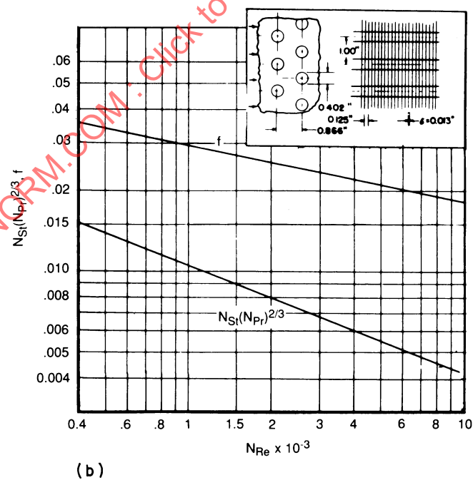
Figure 3H-107 - Finned Circular Tubes; N_{Re} = 4r_h G/\mu
