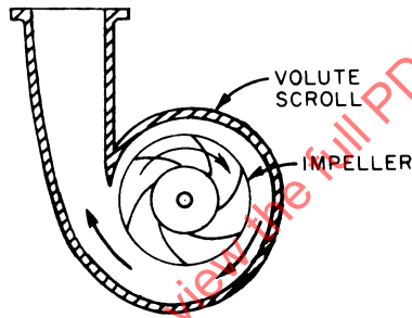
Figure 3H-1 - Volute Pump
