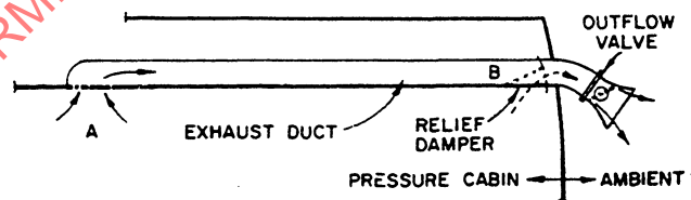
Figure 3E-1 - Low pressure exhaust duct
