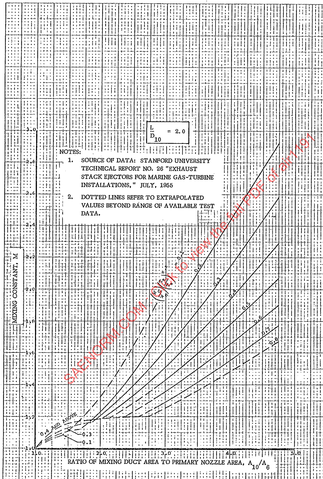
FIGURE 5c. MIXING CONSTANT DATA FOR L/D_{10} = 2.0
