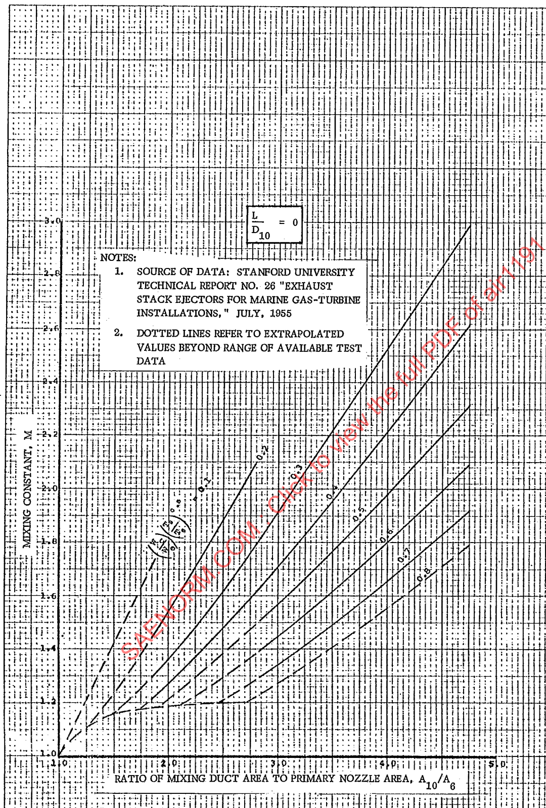
FIGURE 5a. MIXING CONSTANT DATA FOR L/D_{10} = 0
